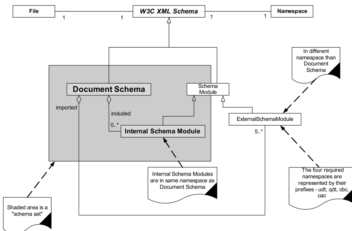
Figure 5. UBL Schema Modularity Model
