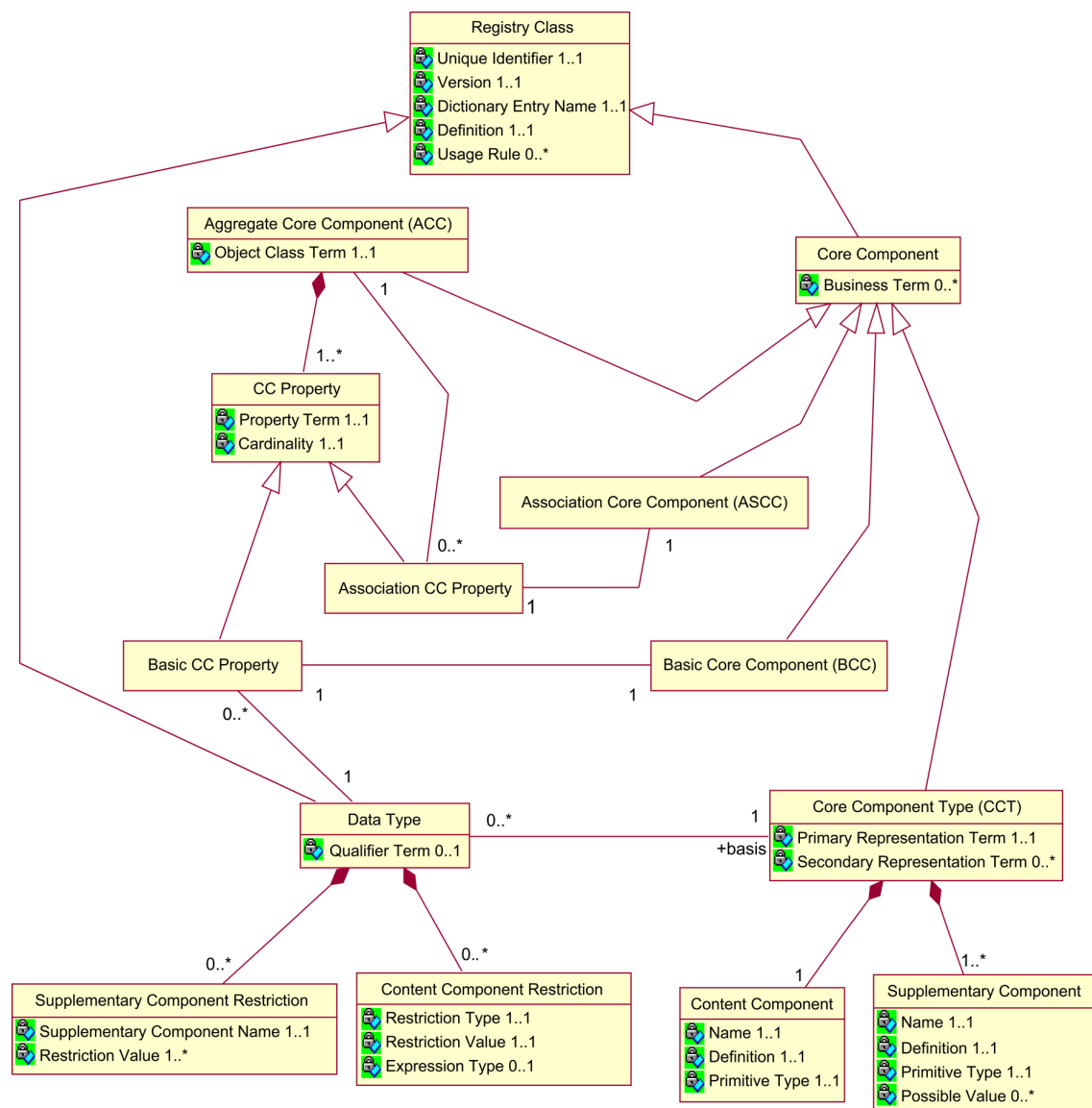
Figure 1. Core Components and Datatypes Metamodel
