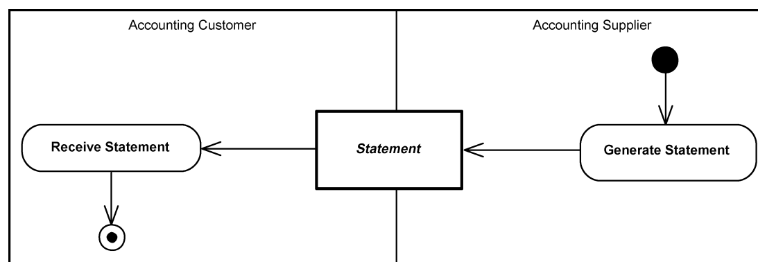
Figure 84. Statement Process
