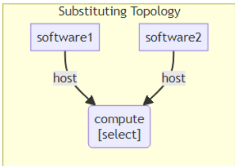
Figure 25: Substituting Template using Selectable Node
