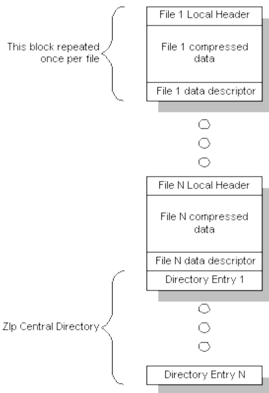
Figure 1 - Zip file structure
