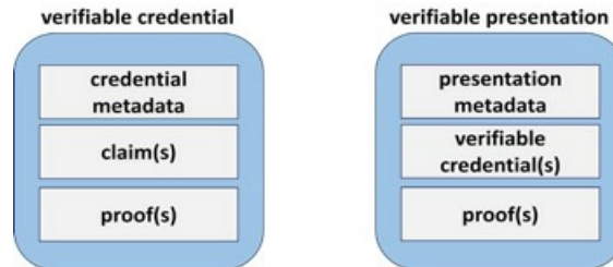
Figure 4: Structure of a VC and a VP
