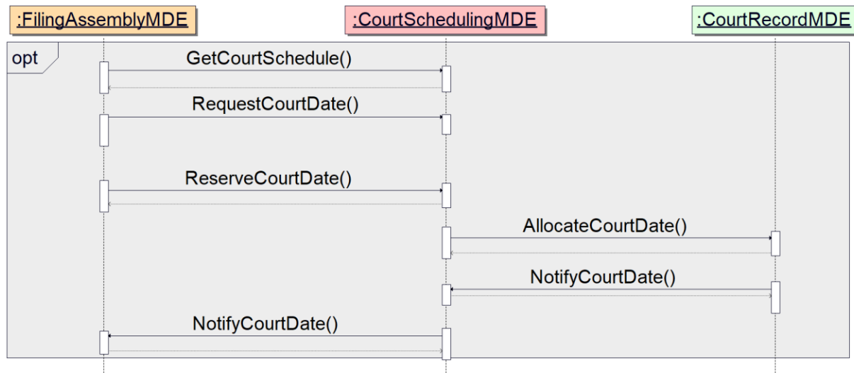
Figure 2. Scheduling Process
