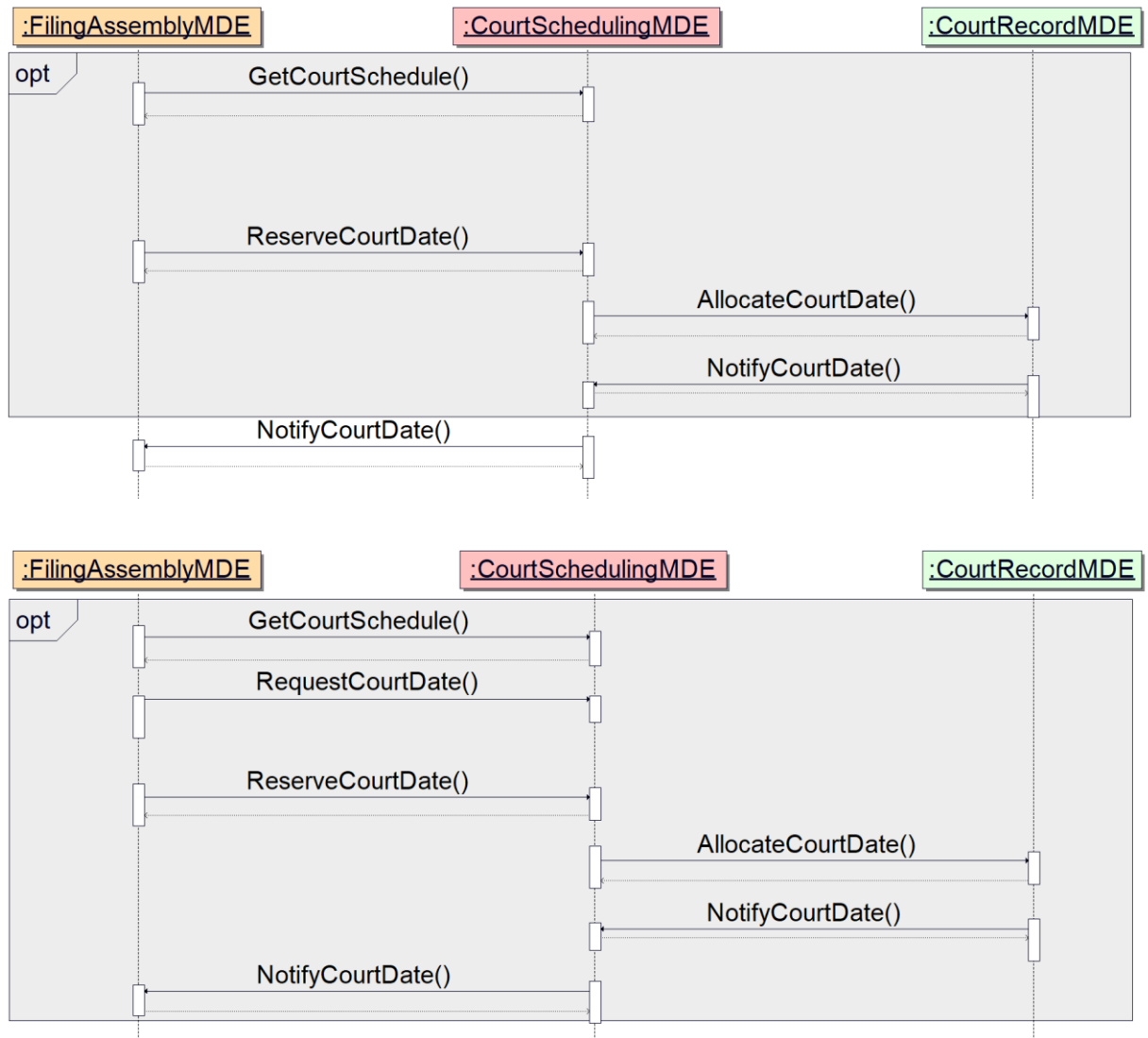
Figure 2-2. Scheduling Process
