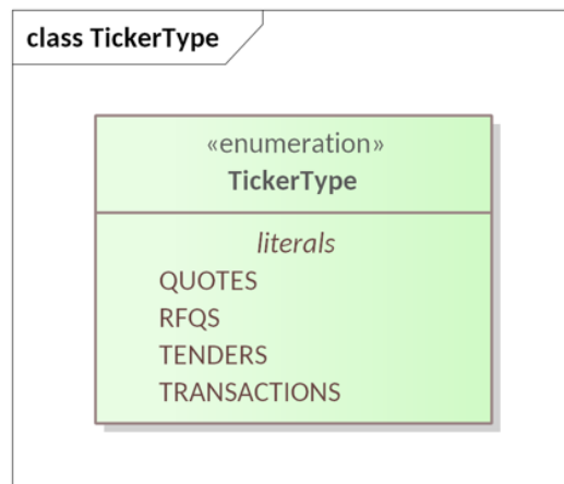
Figure 11-1 TickerType Enumeration
