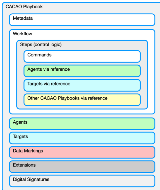
Figure 1--: CACAO Playbook Structure
