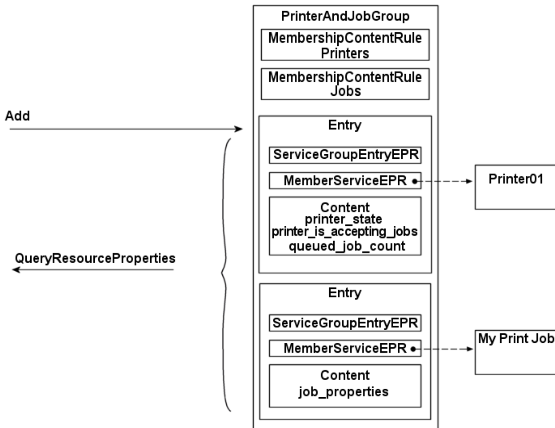
Figure 13: PrinterAndJobGroup resource properties and operations
