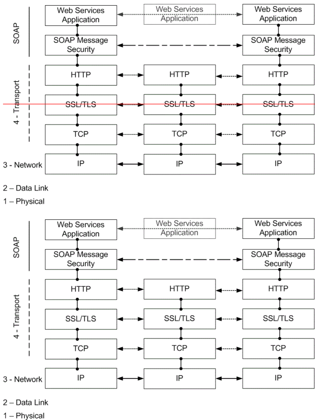
Figure 1: Protocol Stack with SOAP Message Security
