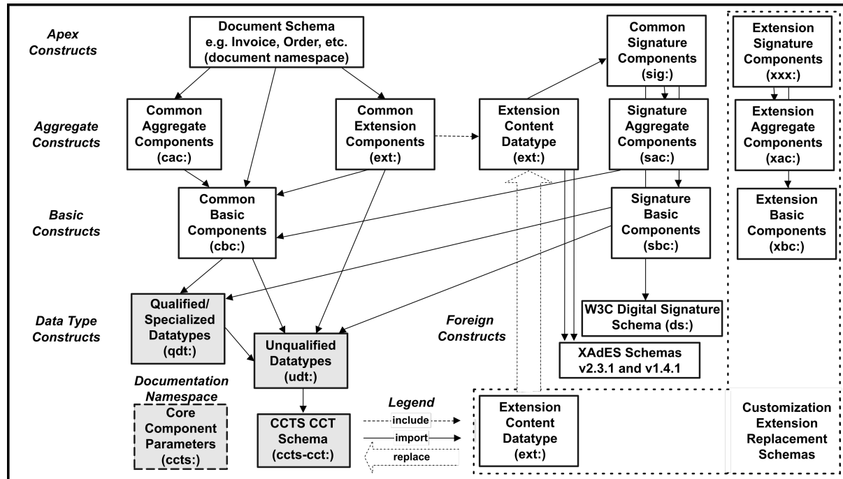
Figure 78. UBL Schema Dependencies
