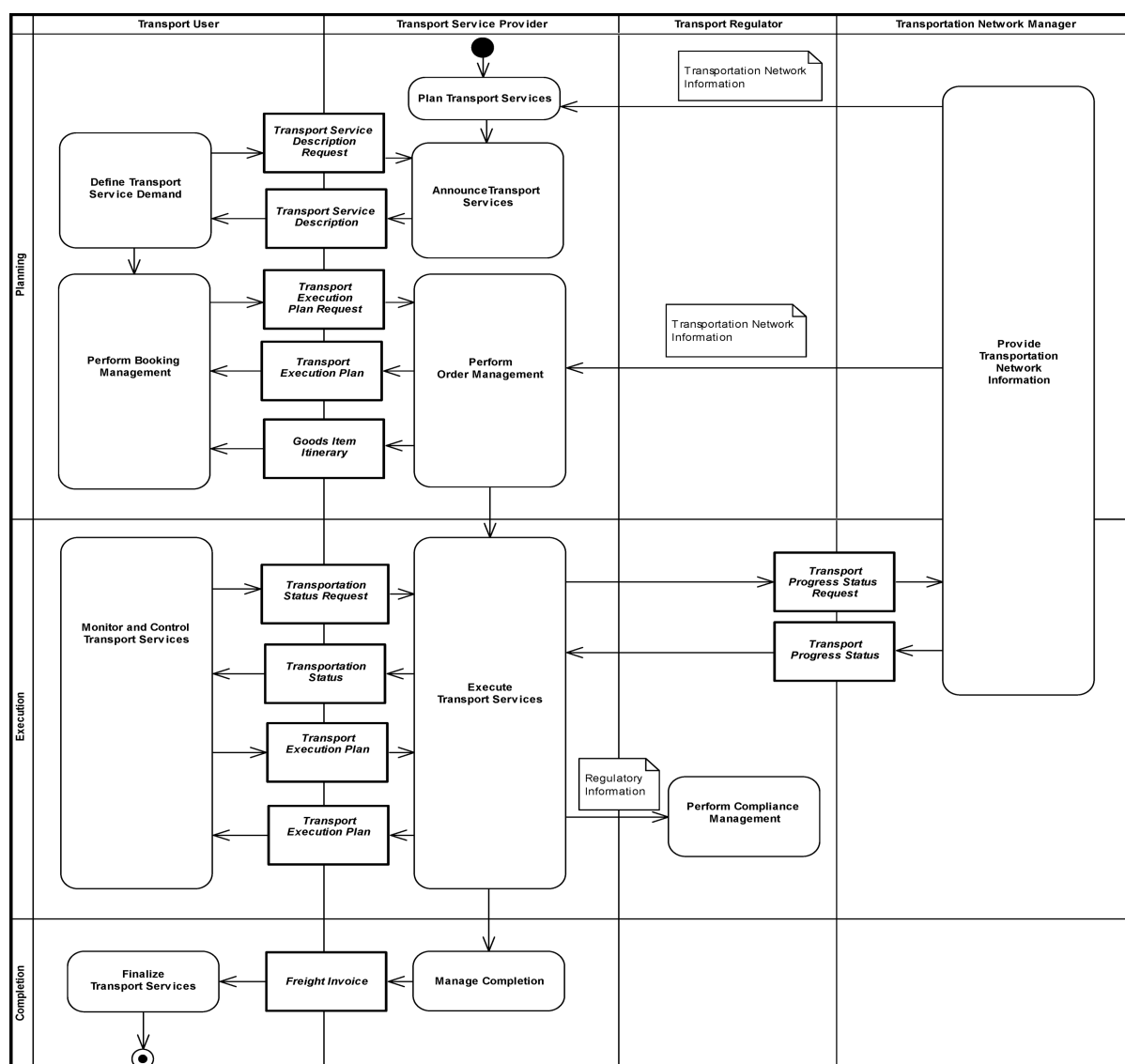
Figure 61. The Intermodal Freight Management Process
