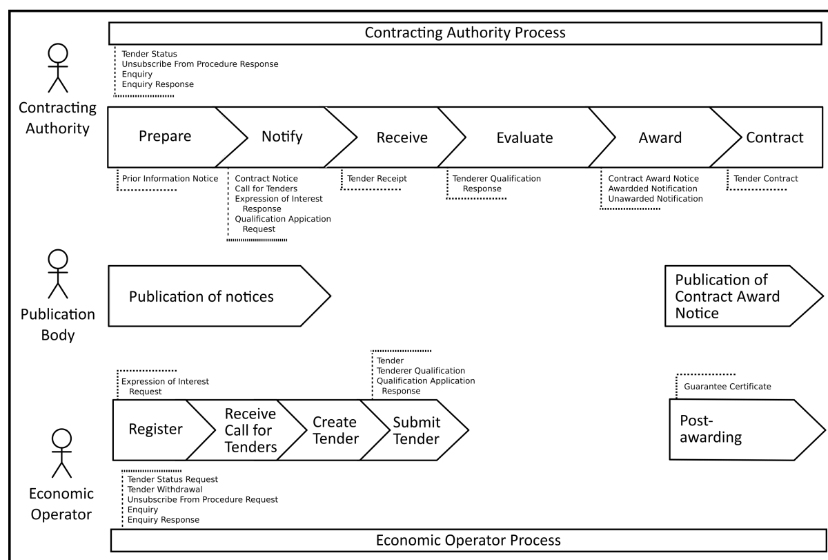
Figure 17. The Tendering Process
