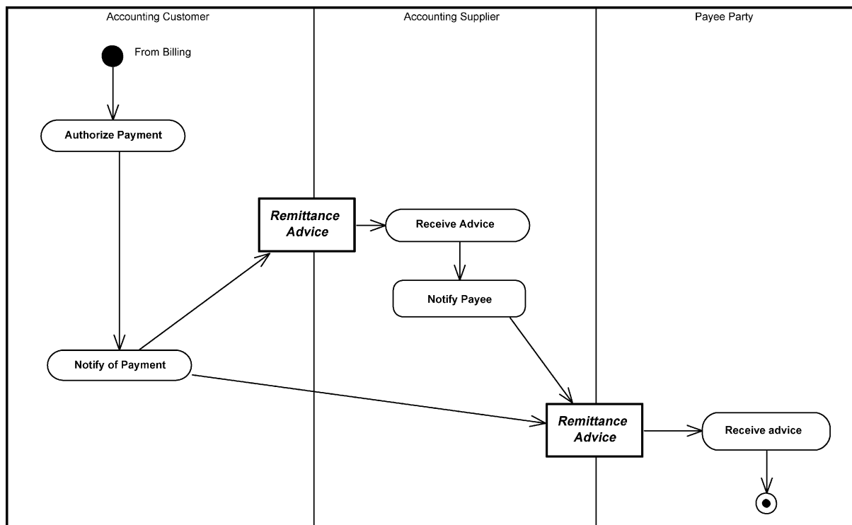
Figure 73. Payment Notification Process
