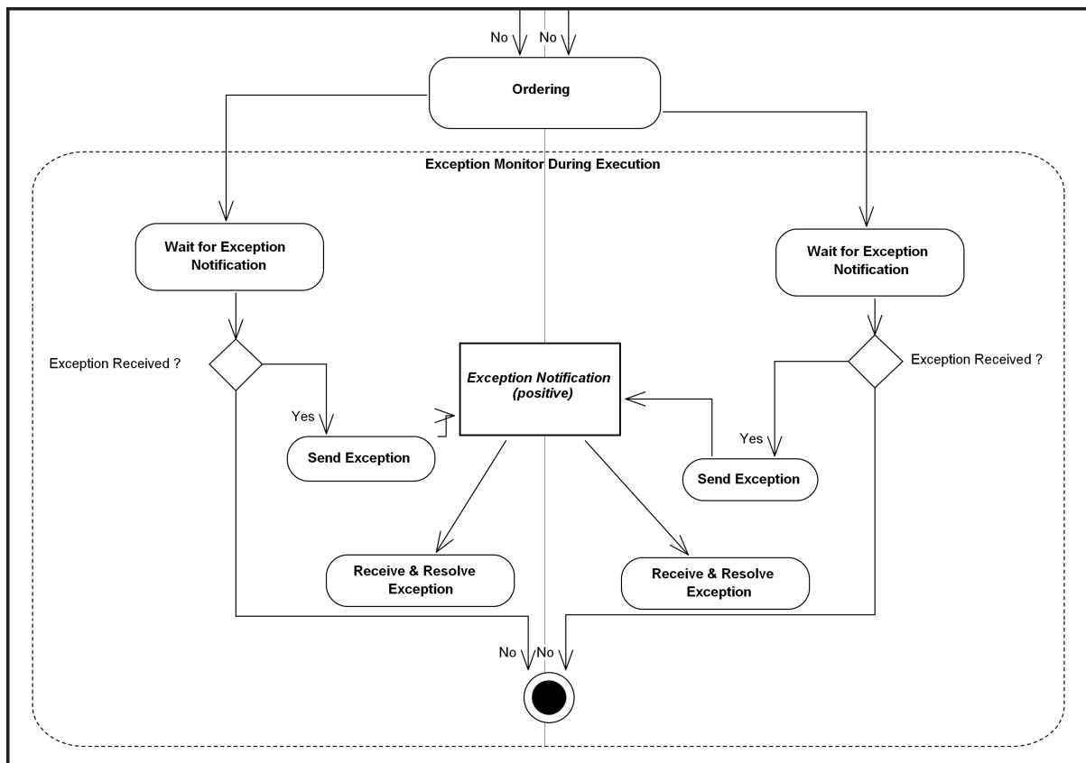
Figure 16. Exception Monitor During Execution
