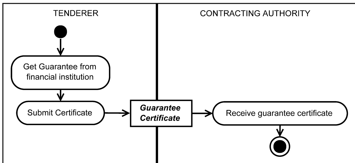
Figure 31. Guarantee Deposit
