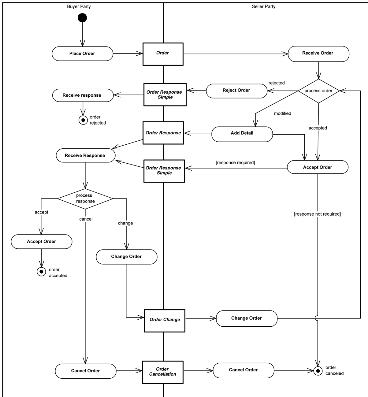
Figure 39. Ordering Process
