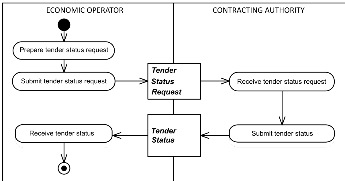
Figure 27. Tender Status
