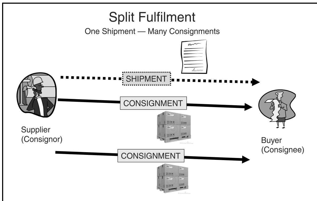
Figure 4. Split Fulfilment
