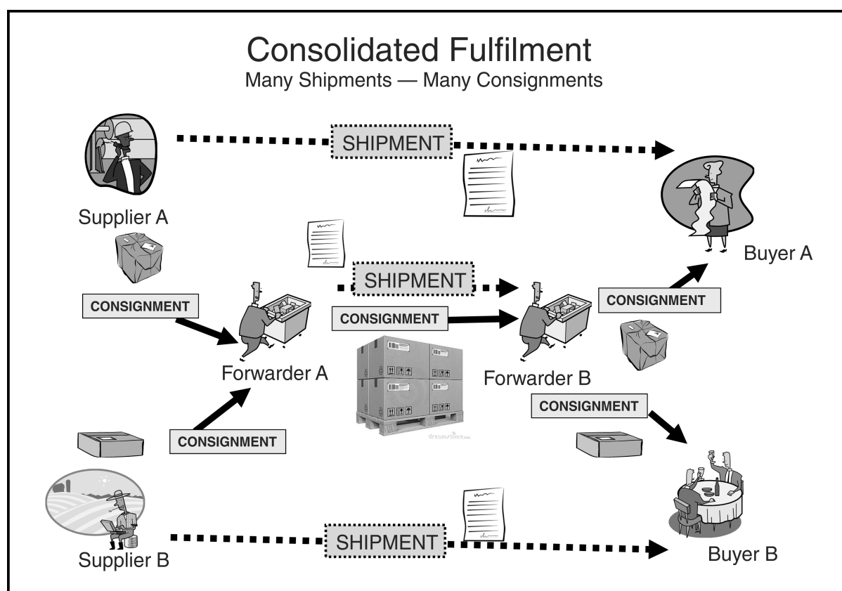
Figure 6. Consolidated Fulfilment
