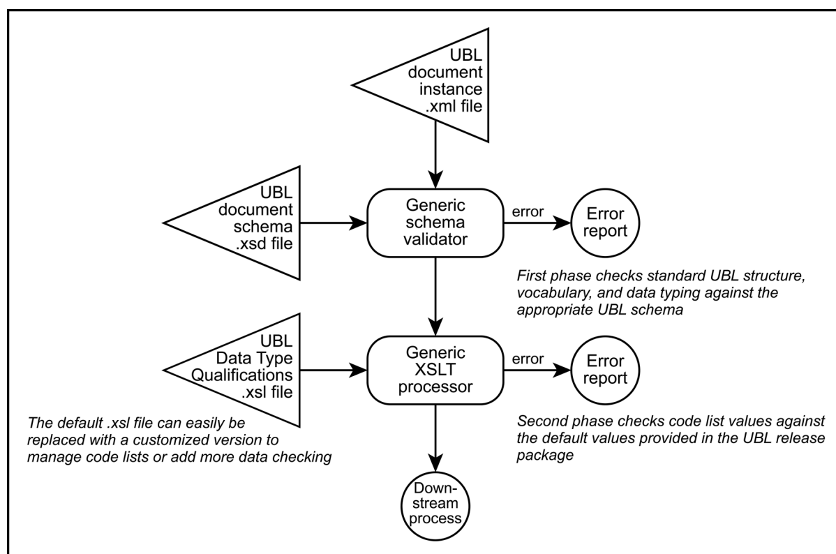
Figure E.2. Two-phase Default UBL 2.2 Validation
