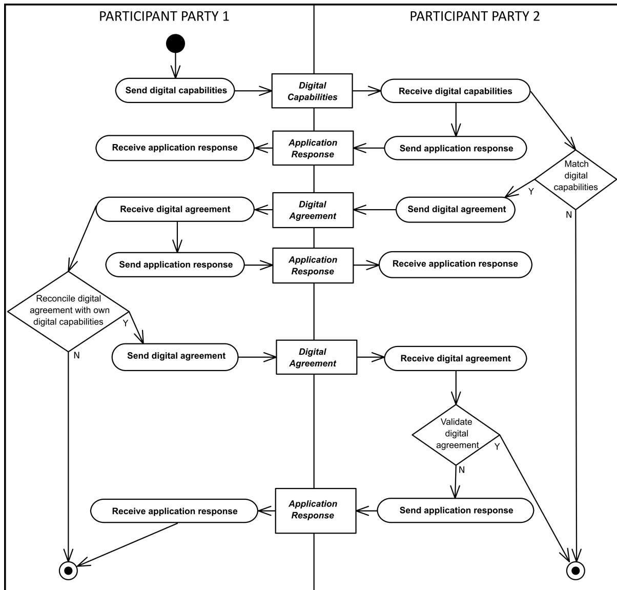
Figure 75. Bi-lateral TPA process
