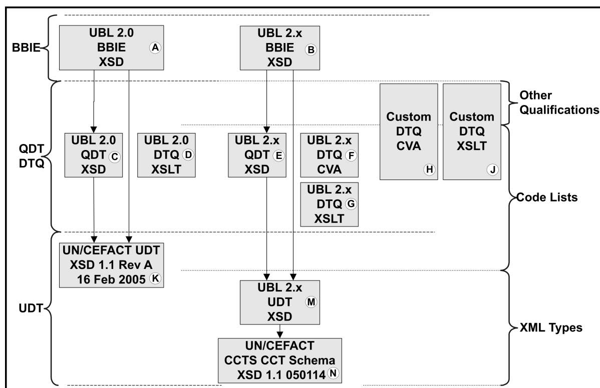
Figure D.1. Data Type Qualification in UBL
