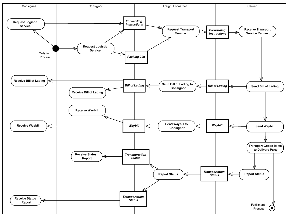
Figure 57. Initiate Freight Management Process
