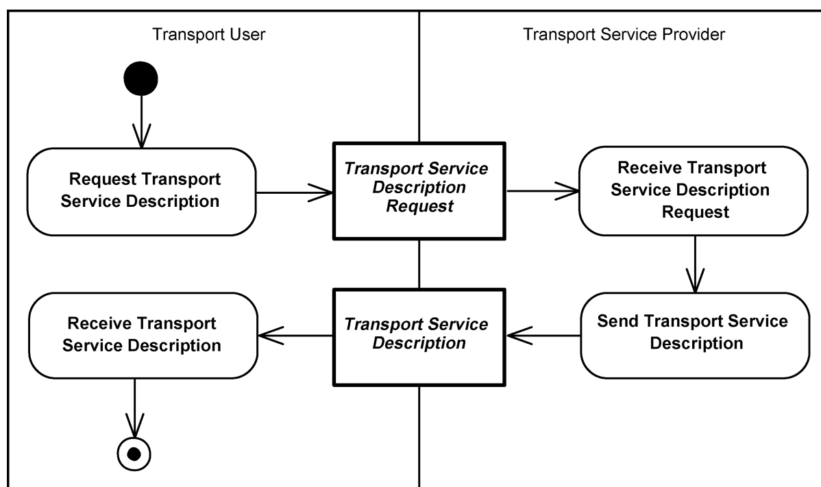
Figure 62. Transport Service Description
