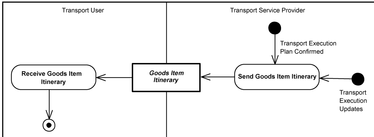
Figure 64. Goods Item Itinerary
