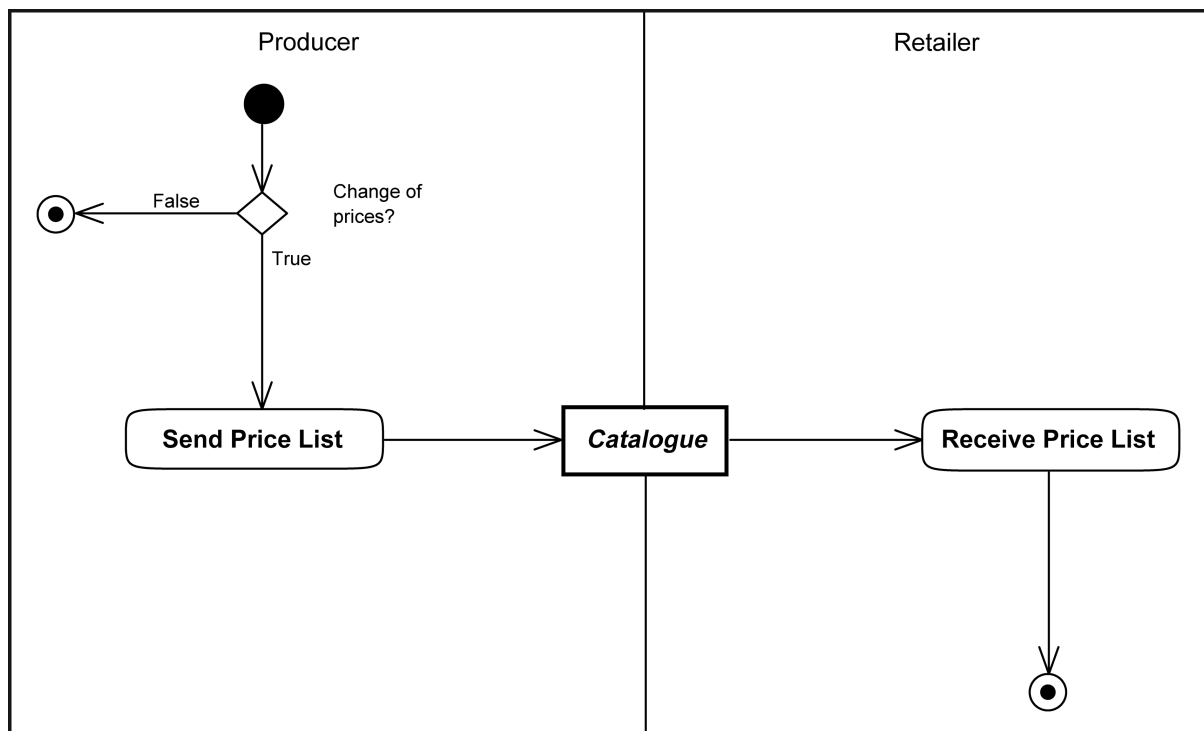
Figure 45. Price Adjustments
