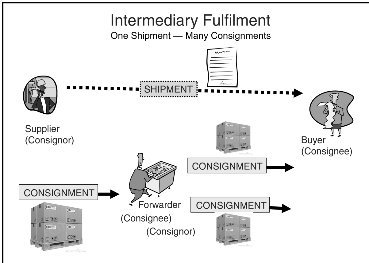
Figure 5. Intermediary Fulfilment
