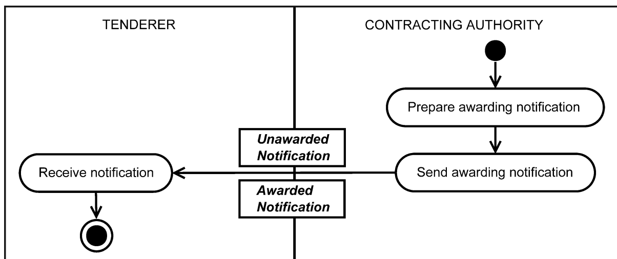
Figure 29. Award Notification
