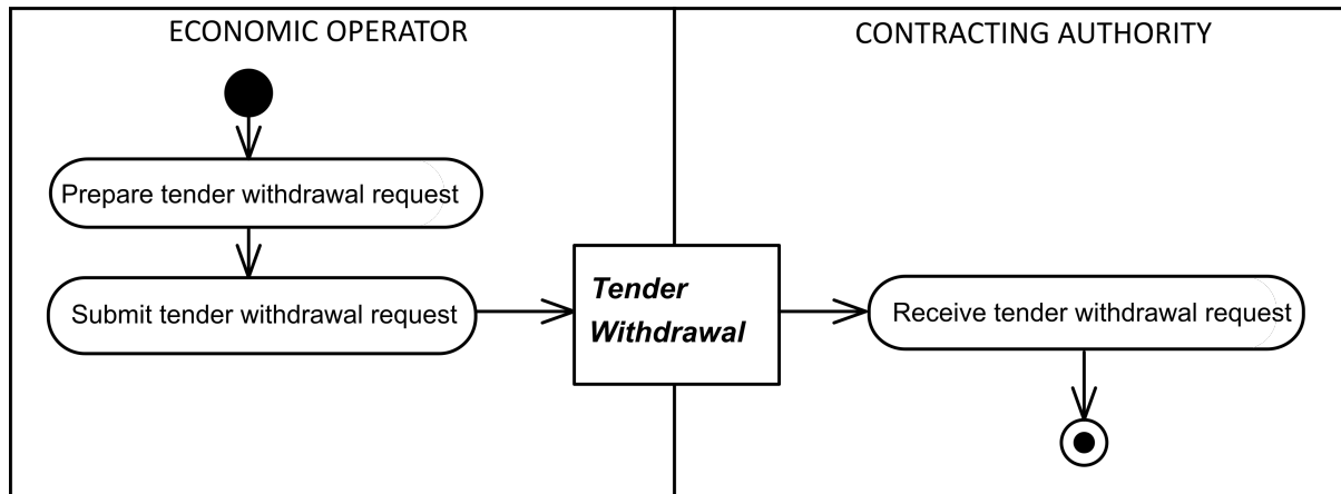
Figure 28. Tender Withdrawal
