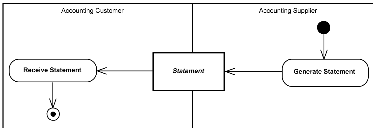
Figure 74. Statement Process
