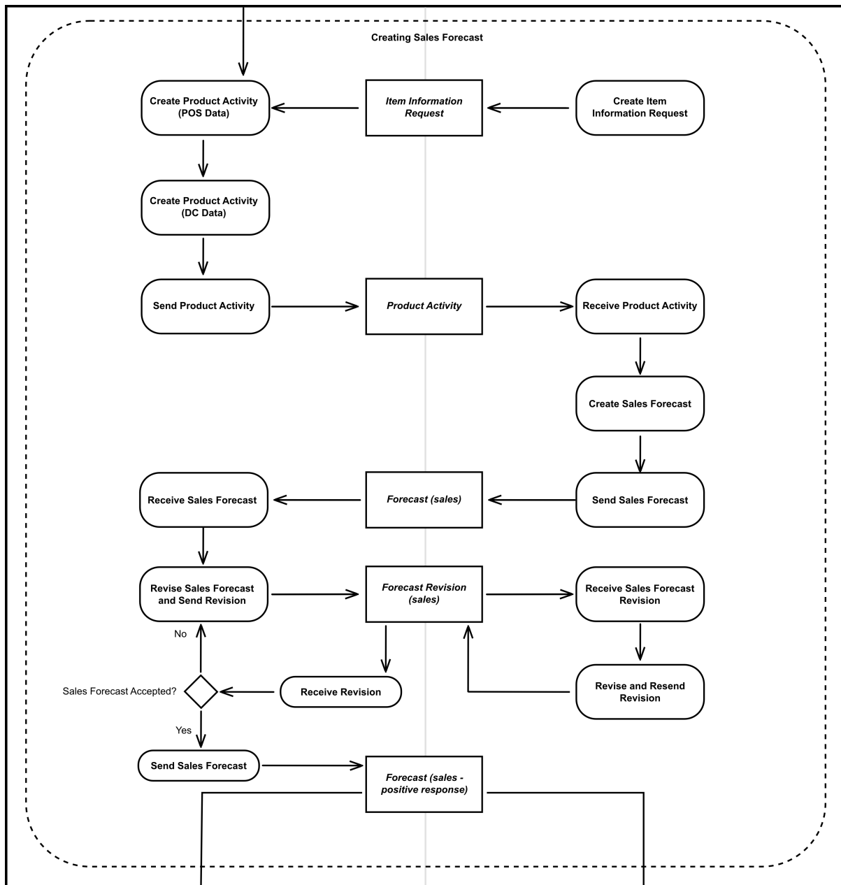
Figure 11. Create Sales Forecast
