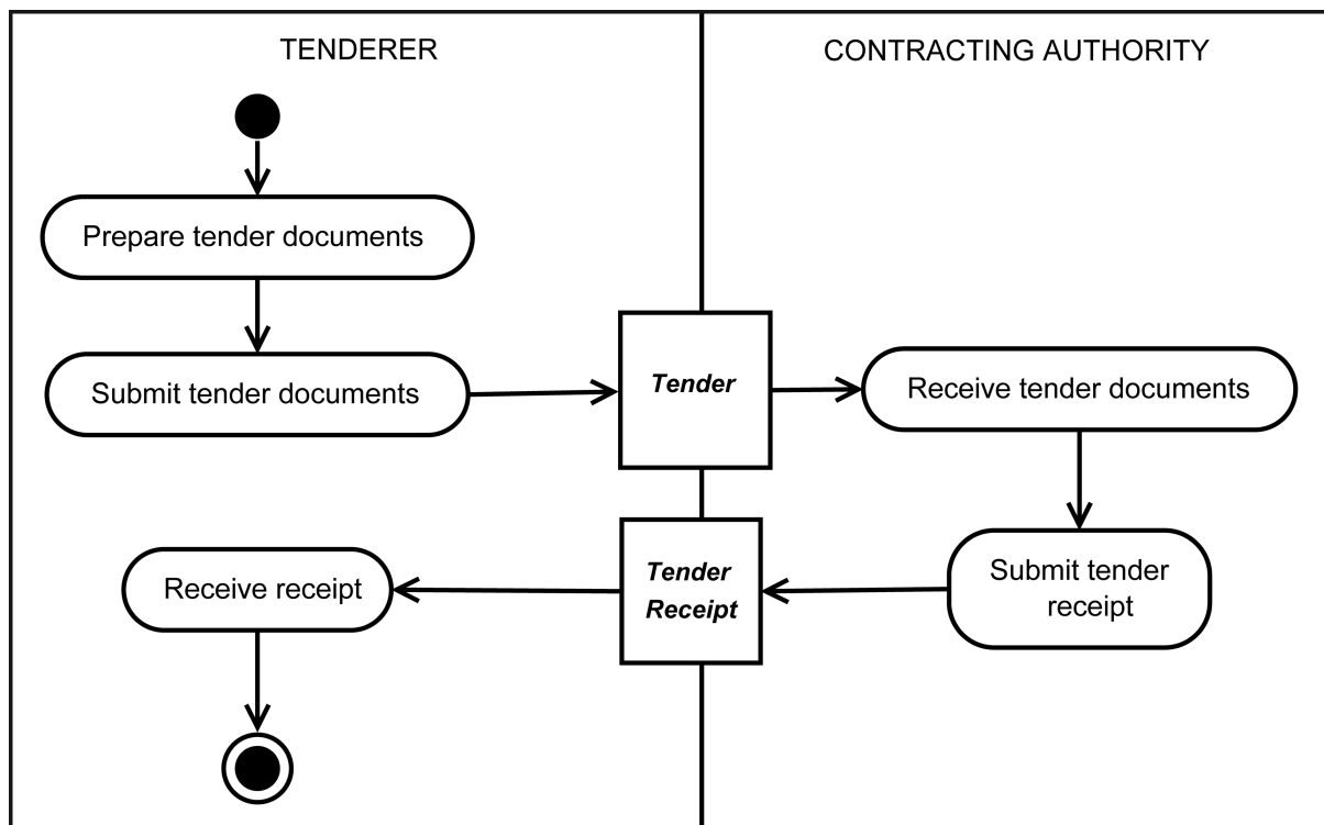
Figure 26. Submission of Tenders
