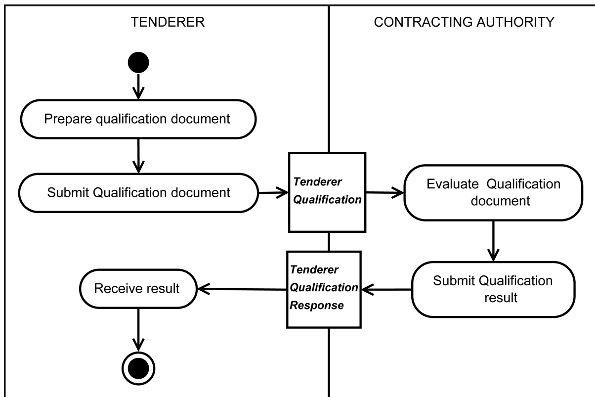
Figure 23. Submission of Qualification Information
