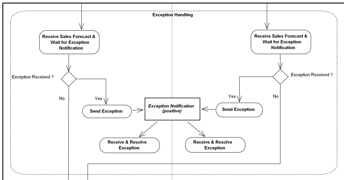
Figure 12. Exception Handling
