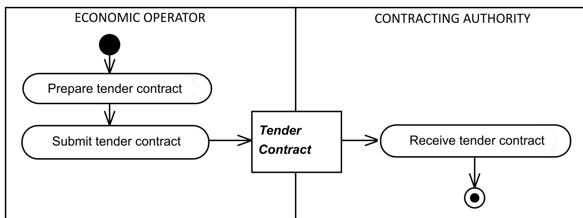
Figure 32. Tender Contract
