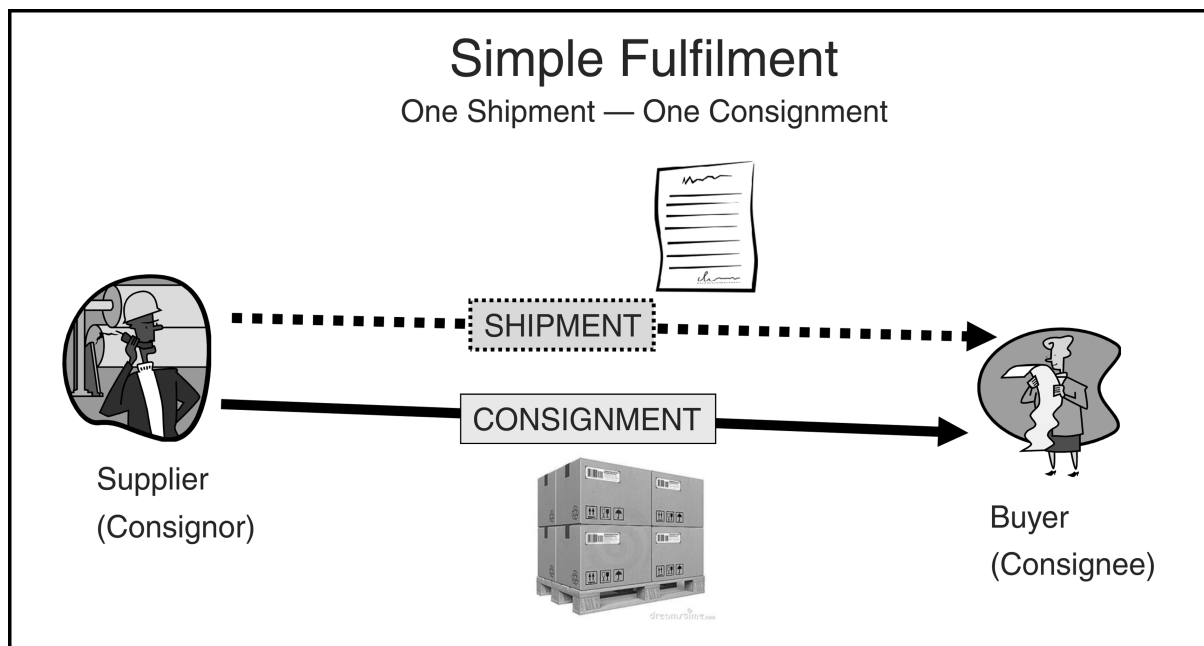
Figure 3. Simple Fulfilment
