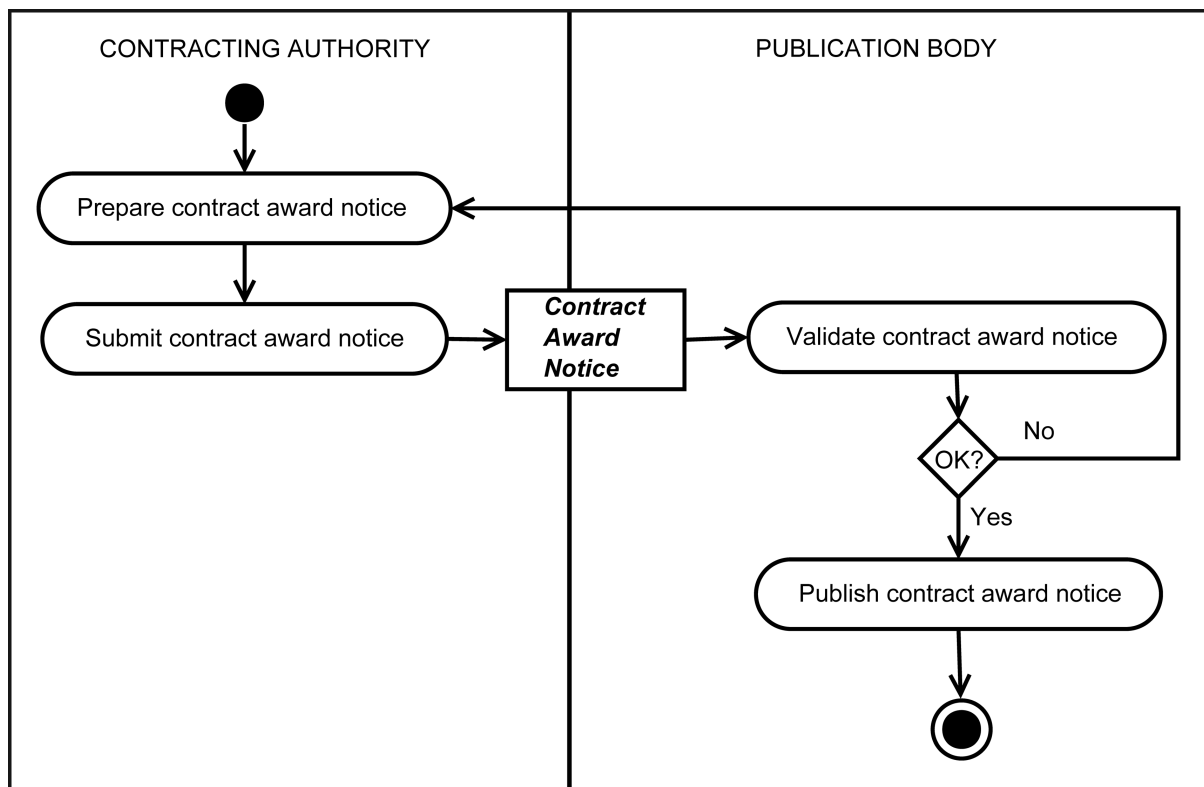
Figure 30. Award Publication
