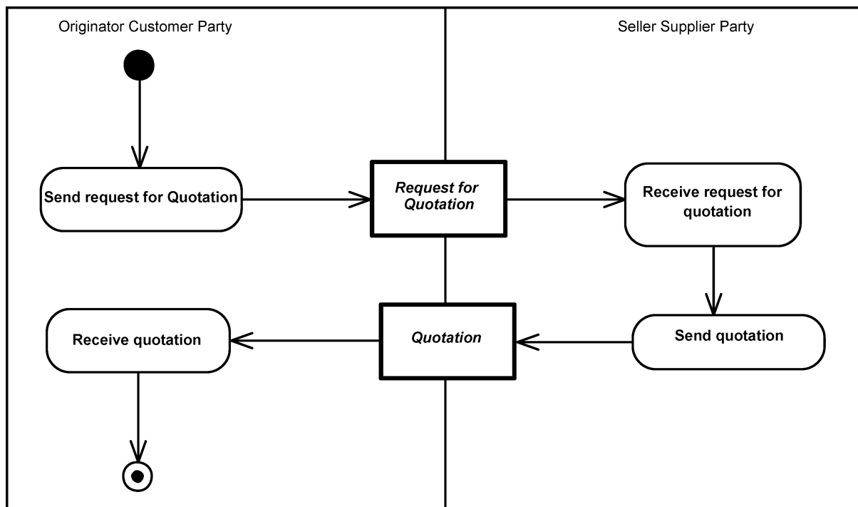
Figure 38. Quotation Process
