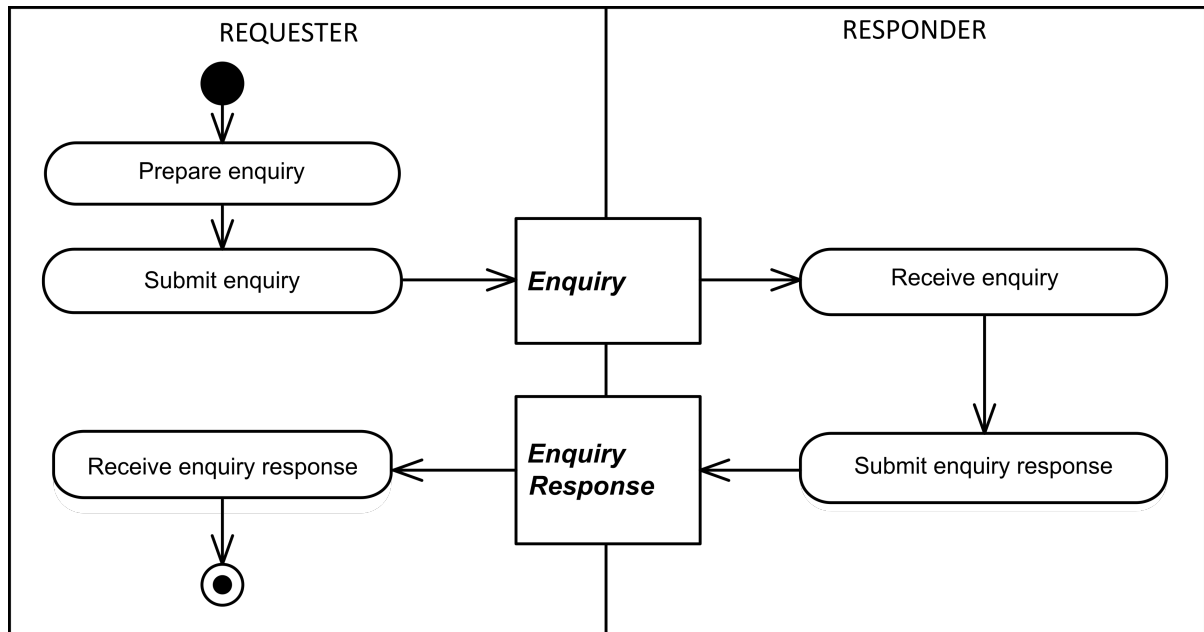
Figure 25. Enquiry
