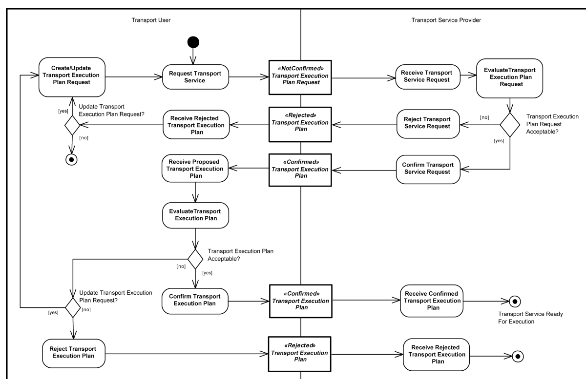
Figure 63. Transport Execution Plan
