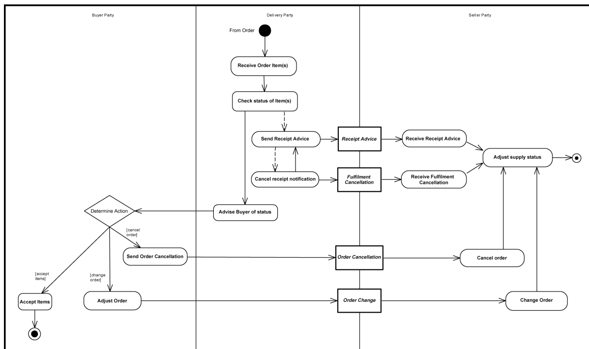
Figure 56. Fulfilment with Receipt Advice
