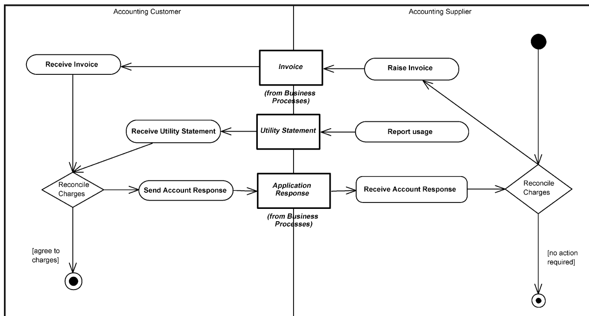
Figure 72. Utility Billing Process
