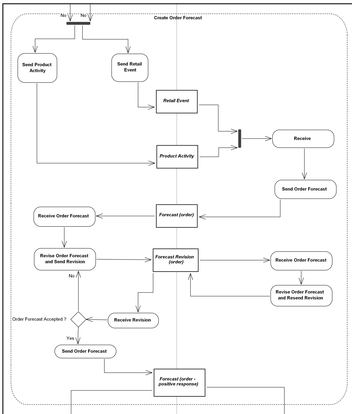
Figure 14. Create Order Forecast
