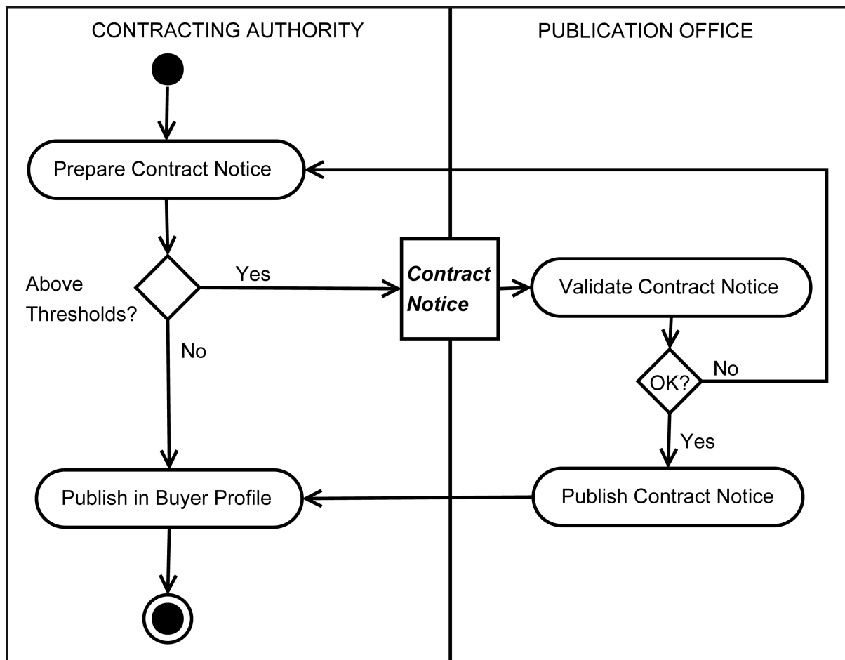
Figure 19. Contract Information Notification
