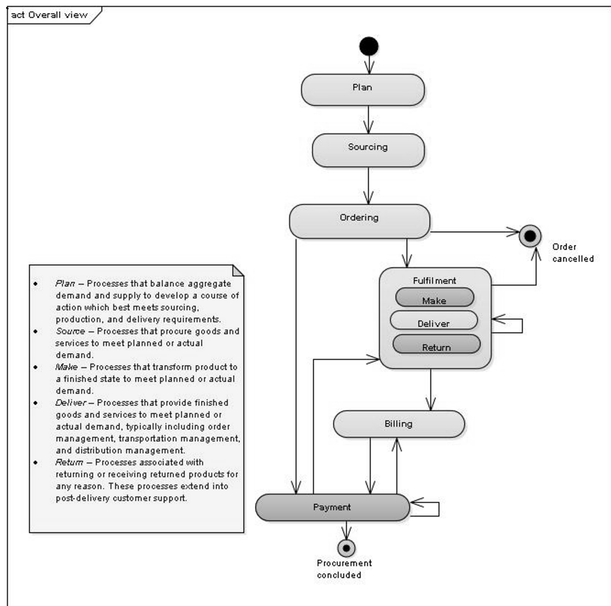
Figure 1. UBL 2.2 Use Case Overall View
