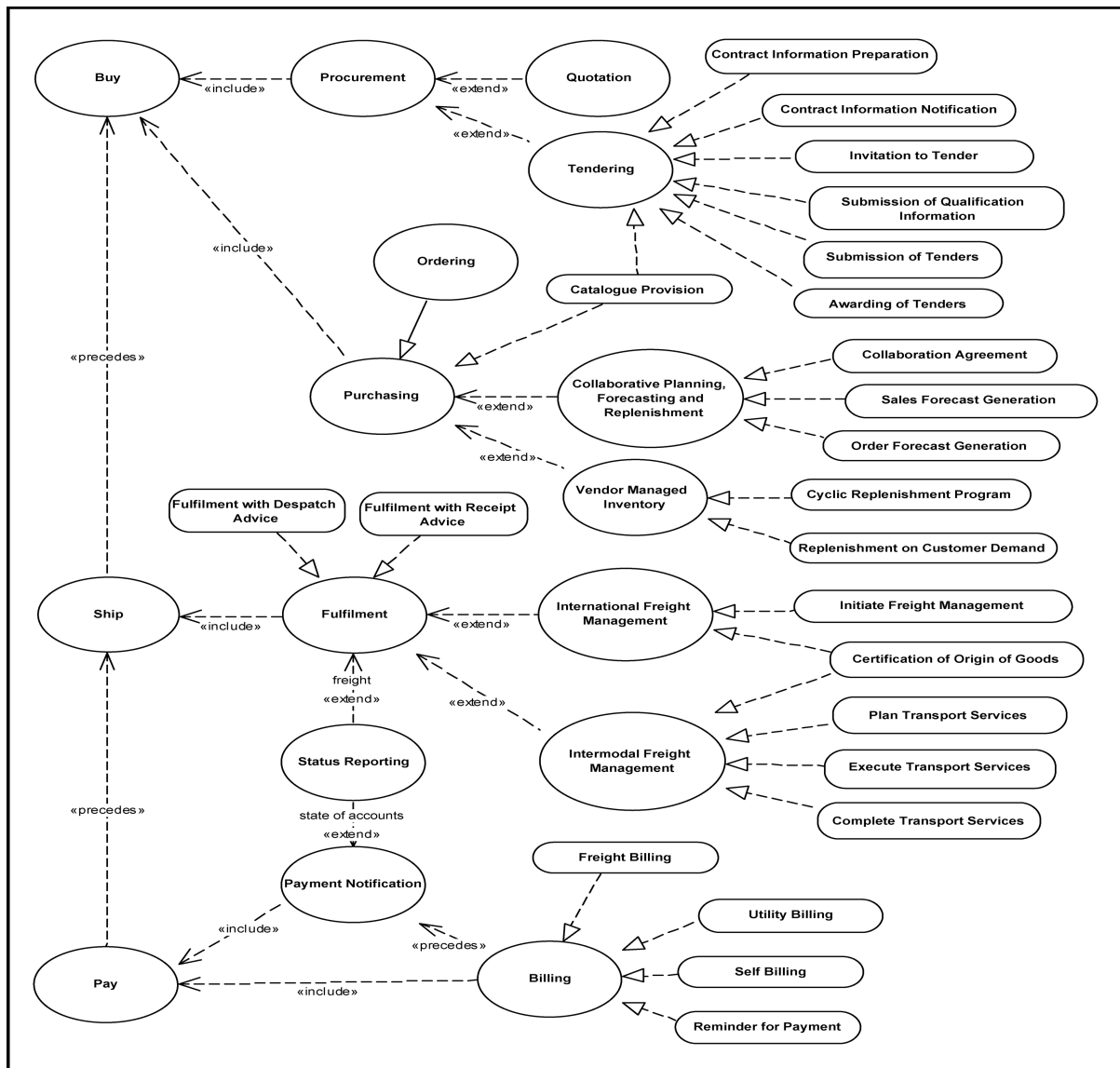
Figure 2. UBL 2.2 Use Case Detail
