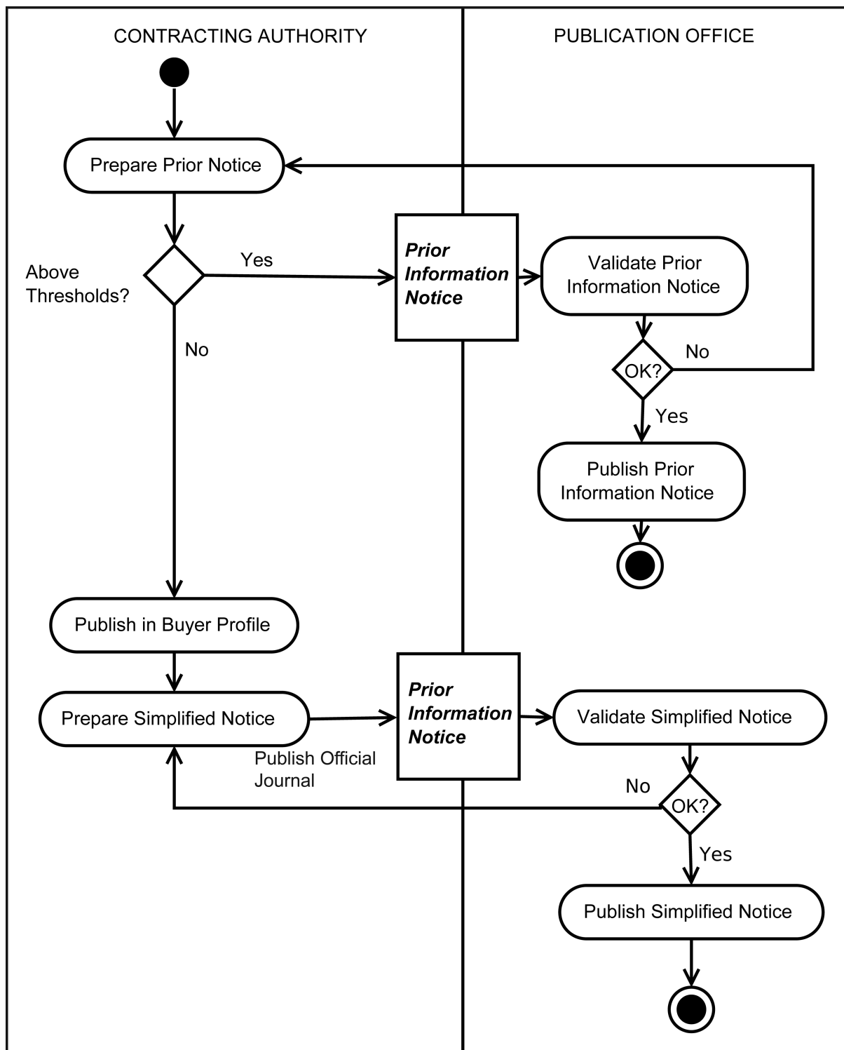
Figure 18. Contract Information Preparation
