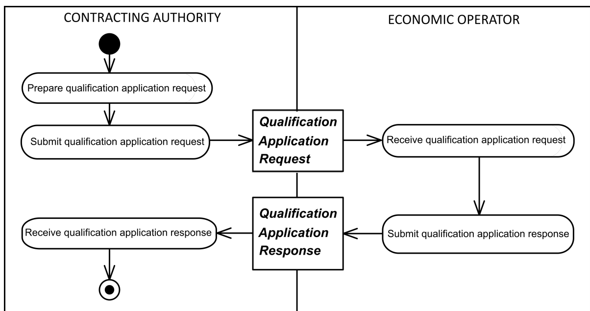
Figure 24. Qualification of Interest
