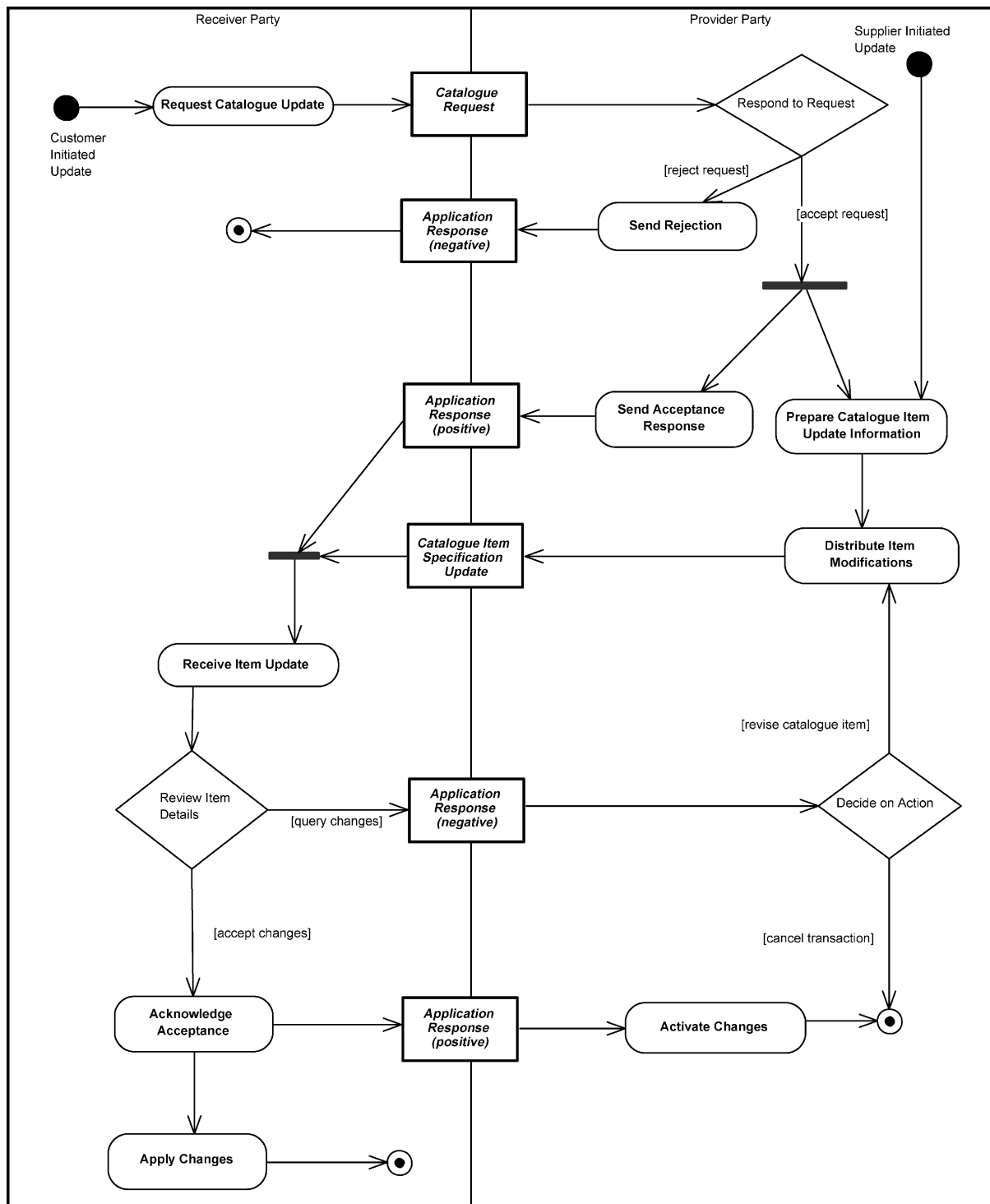
Figure 34. Update Item Specification Process
