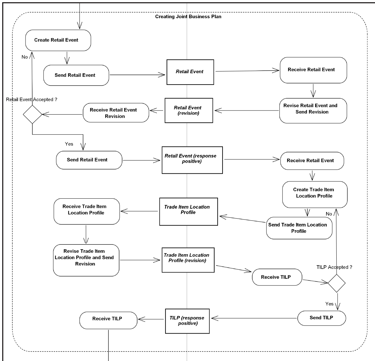
Figure 9. Create Joint Business Plan
