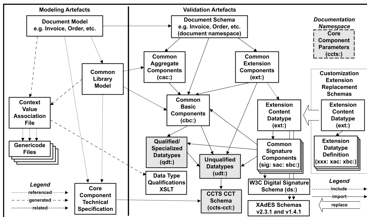
Figure C.1. UBL Data Model Realization
