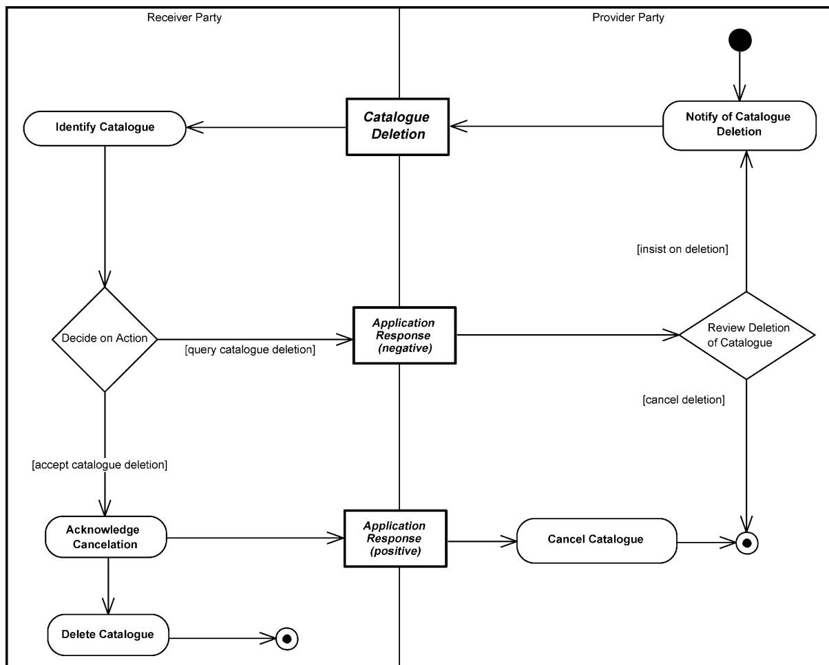
Figure 36. Delete Catalogue Process
