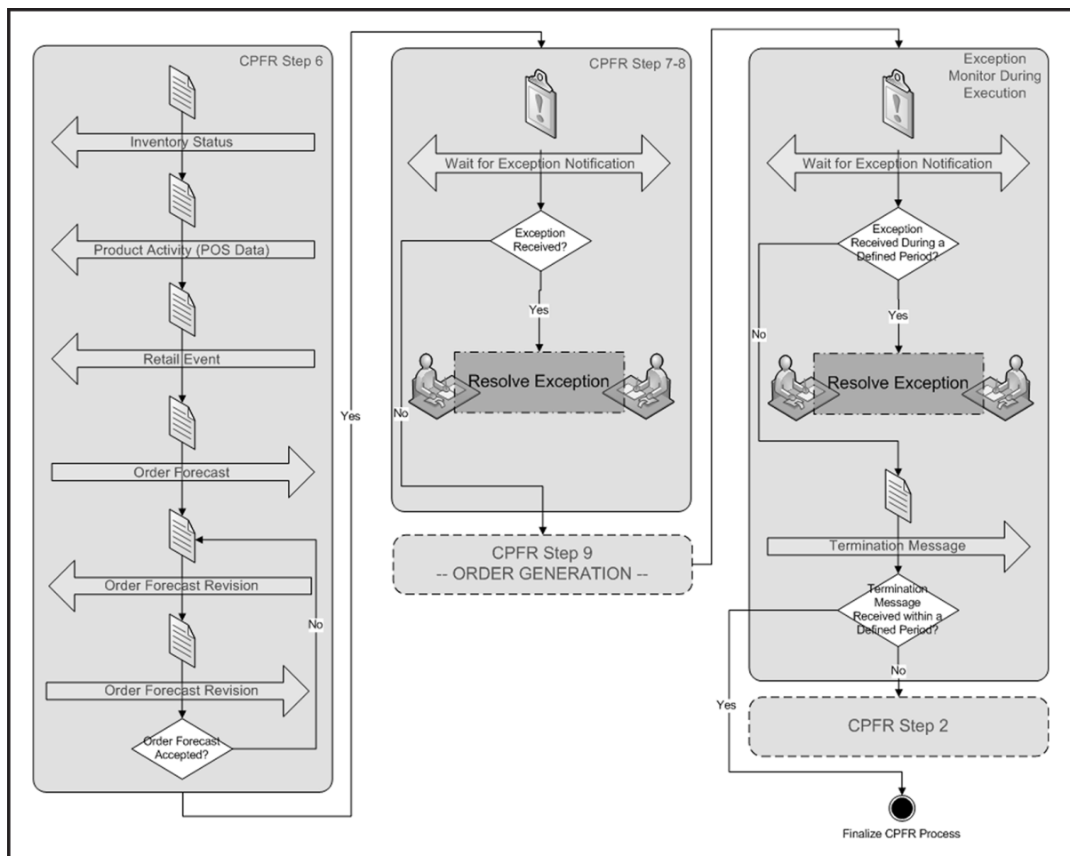
Figure 13. CPFR Steps 6, 7, 8 and 9
