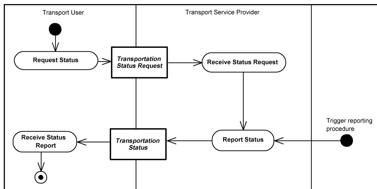
Figure 58. Freight Status Reporting Process
