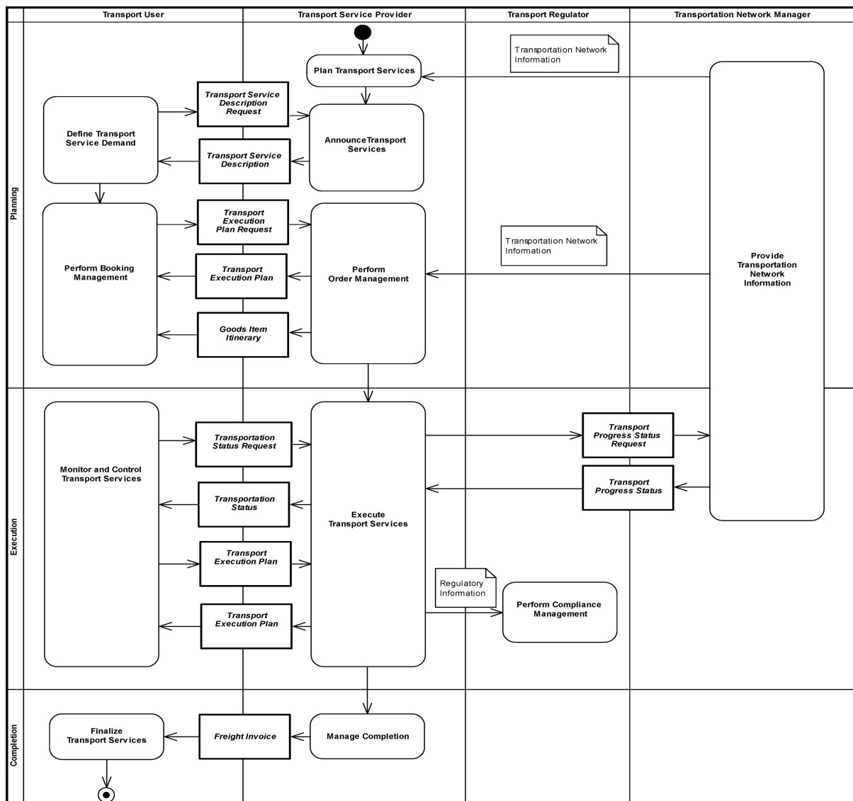
Figure 61. The Intermodal Freight Management Process
