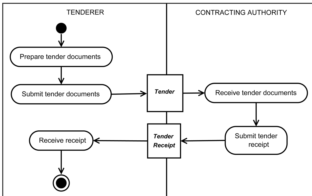
Figure 26 — Submission of Tenders
