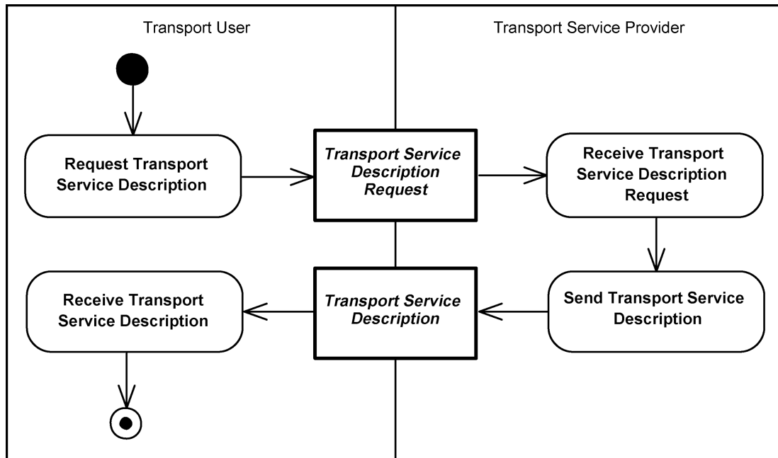
Figure 62 — Transport Service Description
