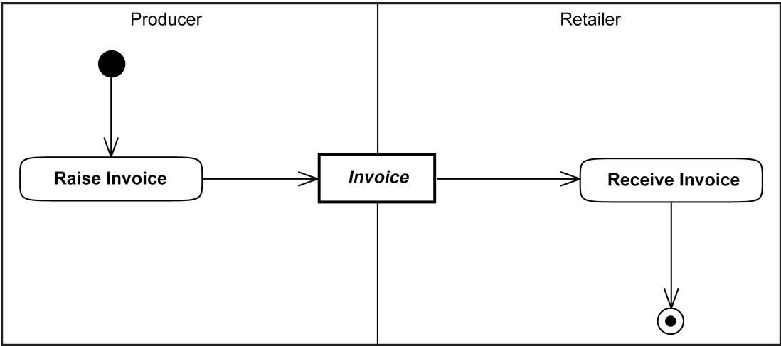
Figure 49 — Invoicing for Cyclic Replenishment Program
