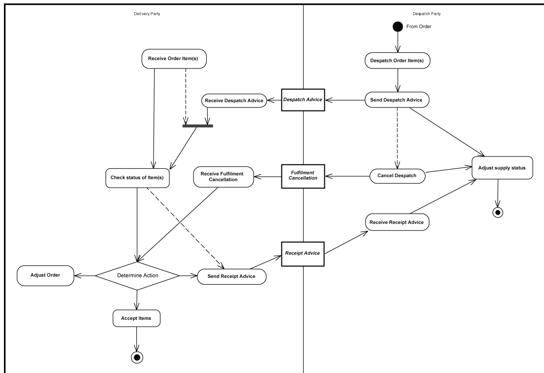
Figure 55 — Fulfilment with Despatch Advice
