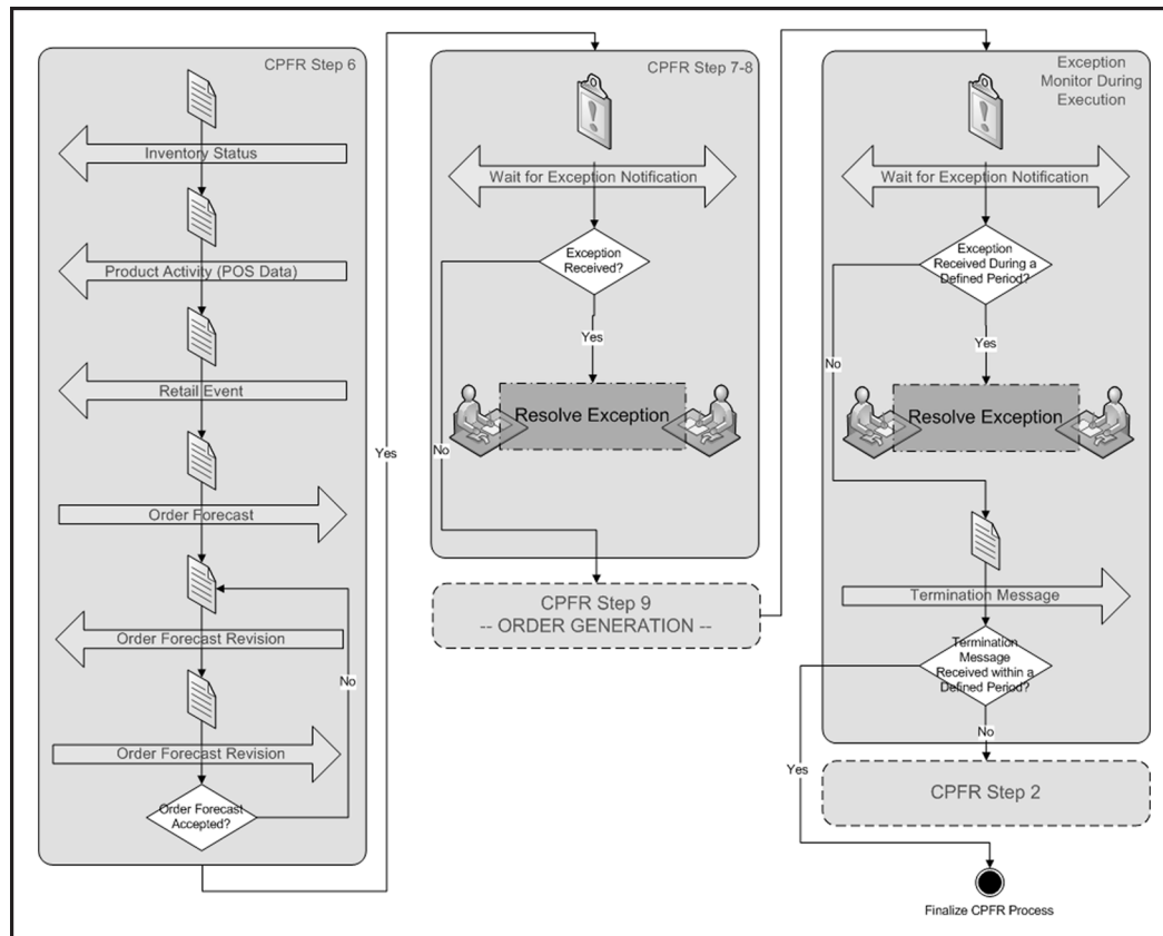
Figure 13 — CPFR Steps 6, 7, 8 and 9
