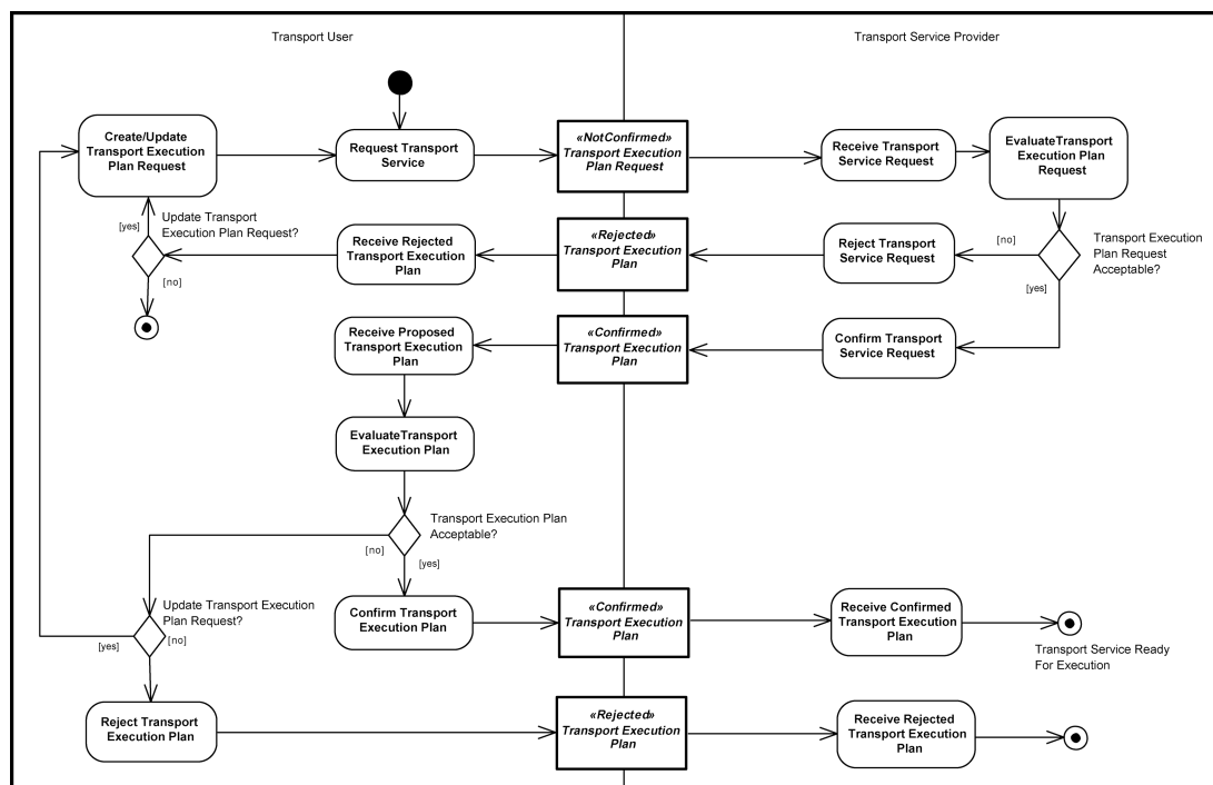
Figure 63 — Transport Execution Plan
