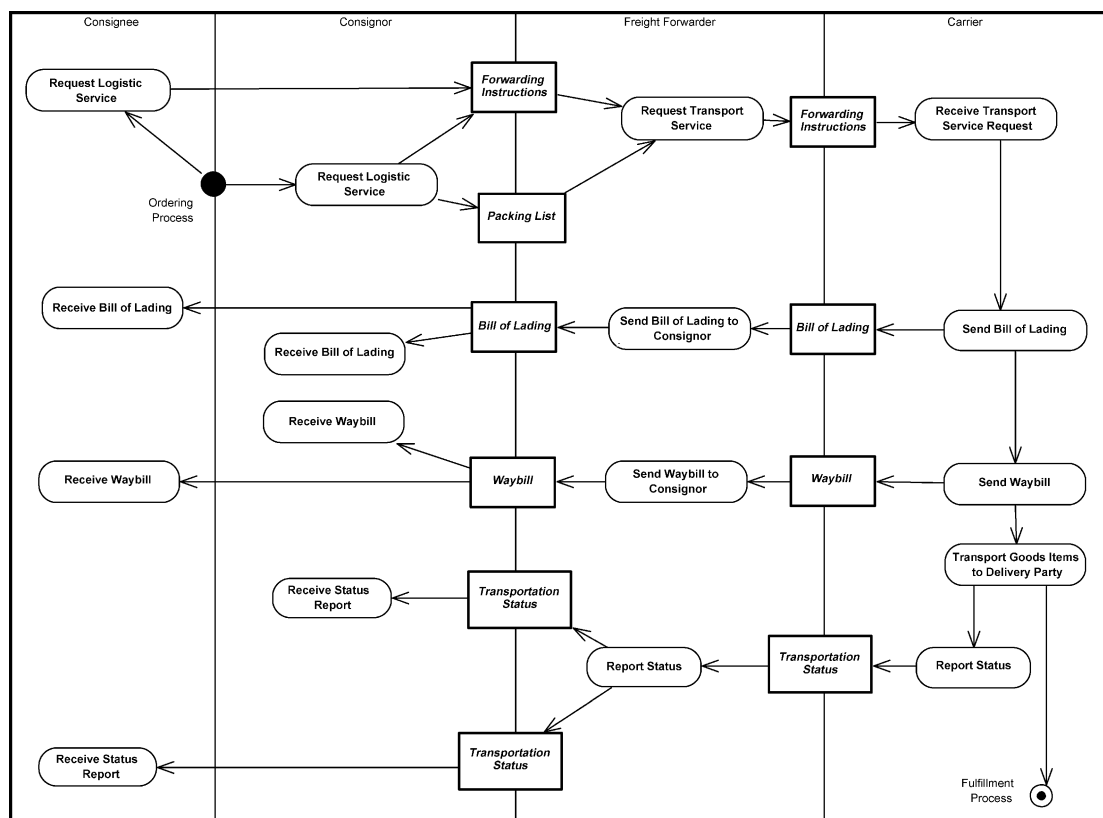
Figure 57 — Initiate Freight Management Process
