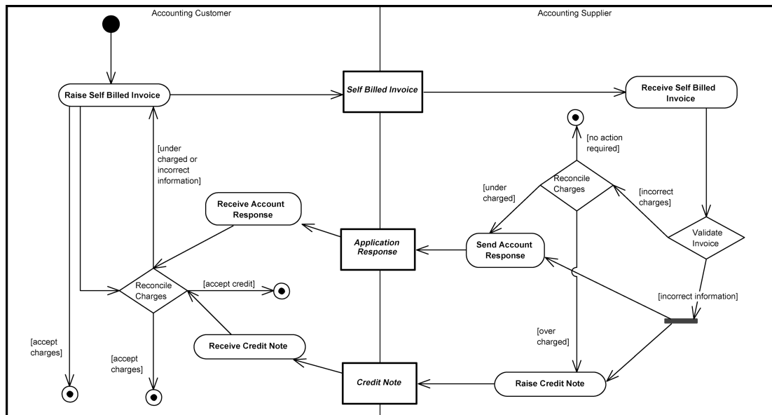
Figure 68 — Self Billing with Credit Note Process
