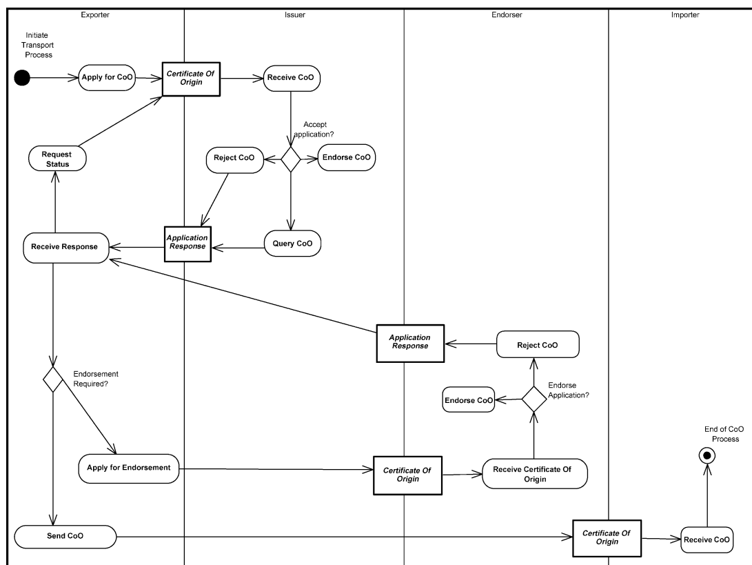
Figure 59 — Certification of Origin of Goods Process
