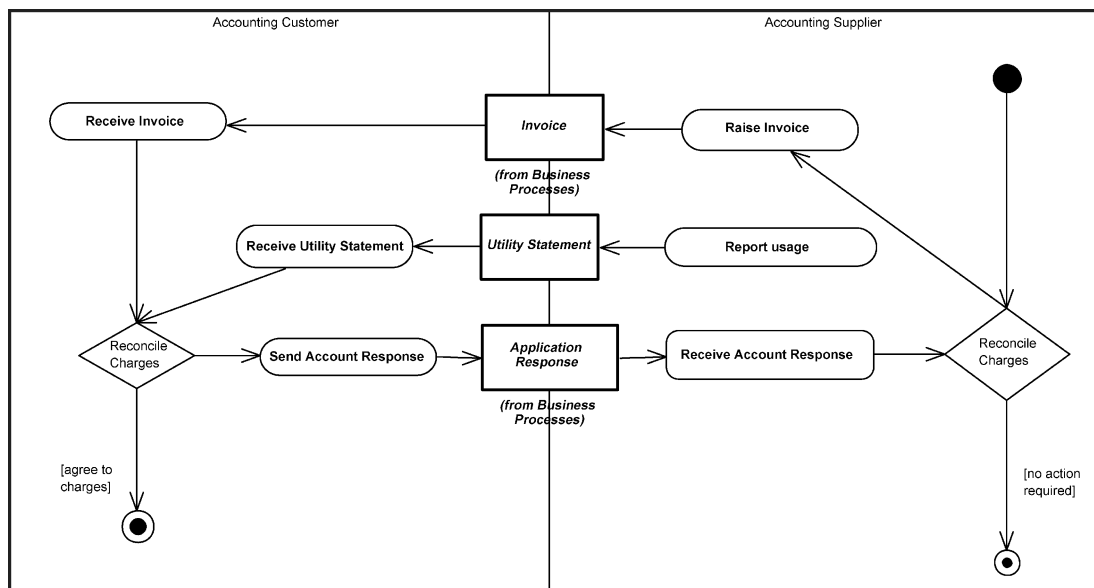
Figure 72 — Utility Billing Process
