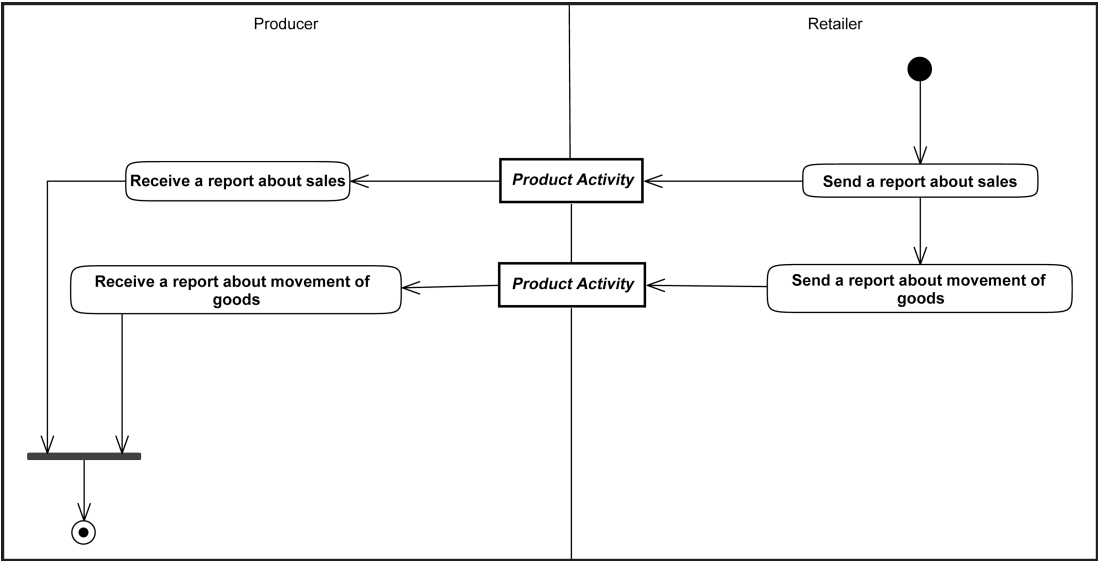
Figure 48 — Report of Sales and Inventory Movements
