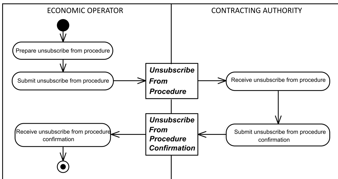
Figure 22 — Unsubscribe from Procedure
