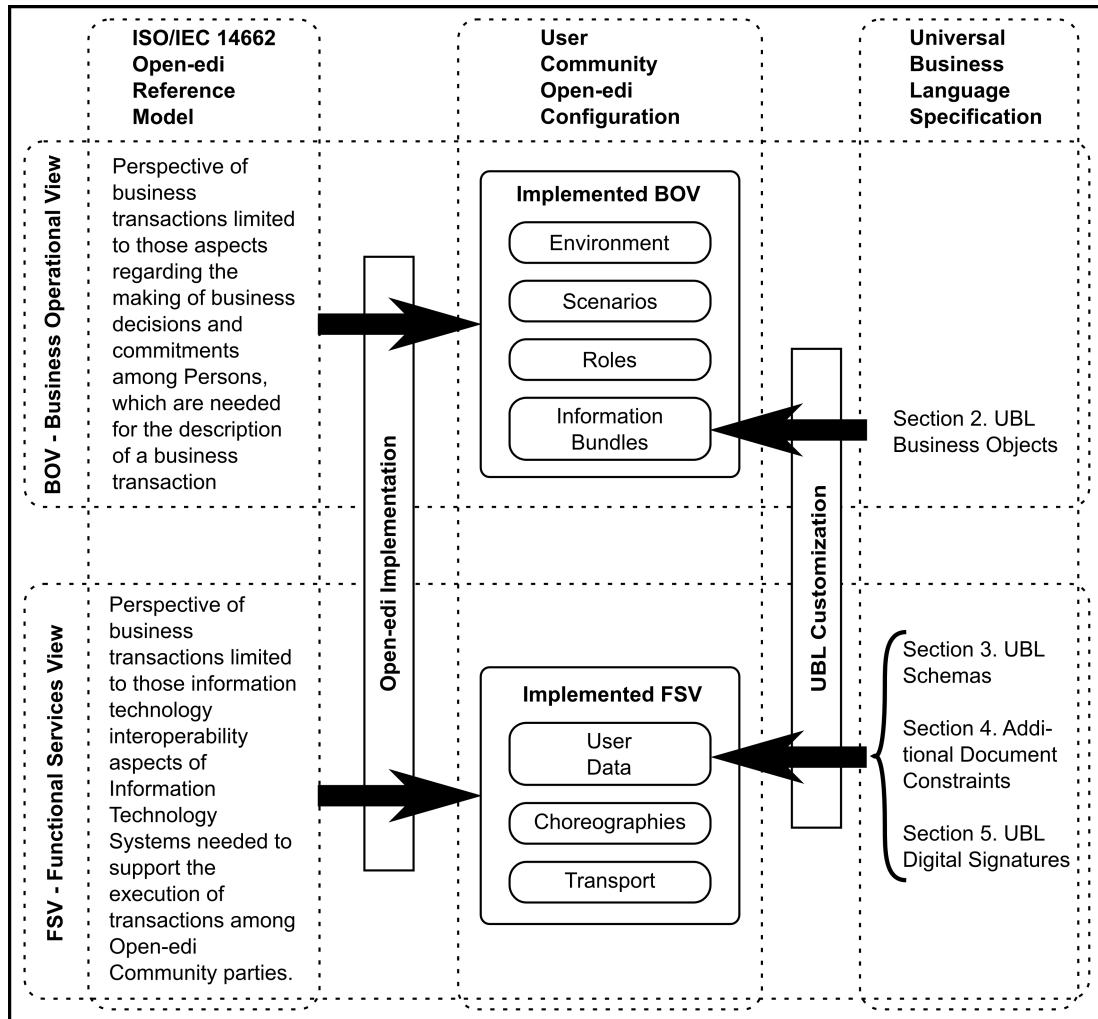
Figure H.2 — Open-edi Application
