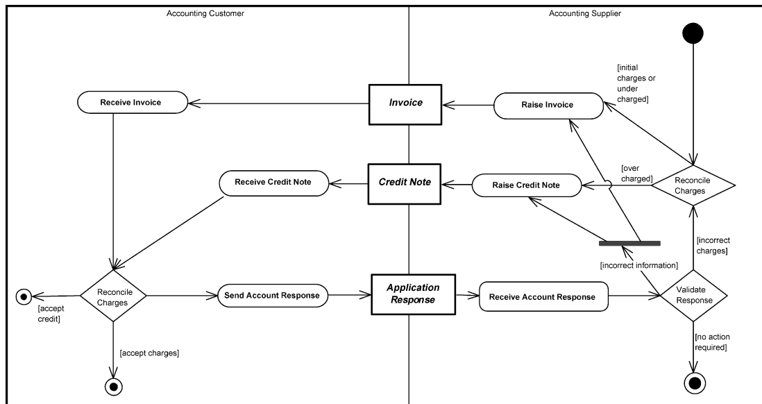
Figure 66 — Billing with Credit Note Process
