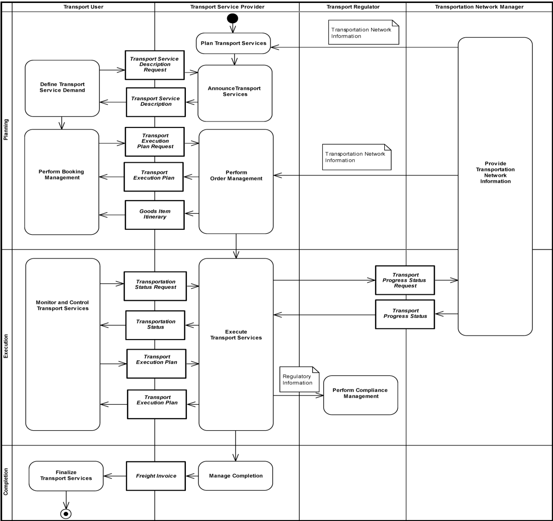
Figure 61 — The Intermodal Freight Management Process
