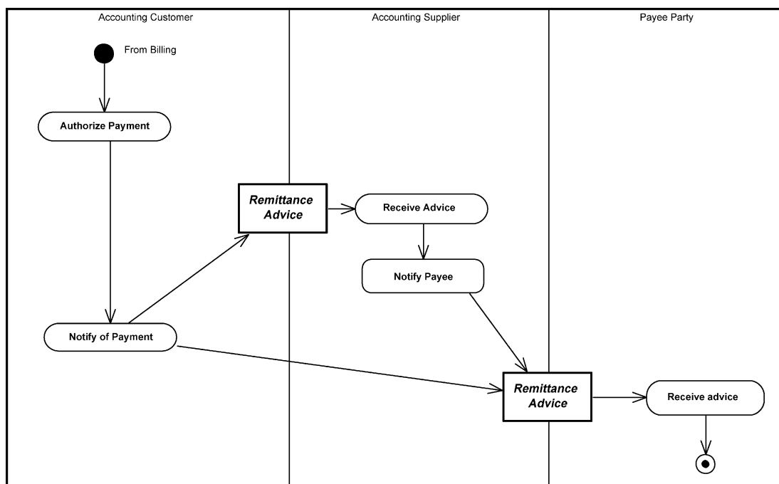
Figure 73 — Payment Notification Process
