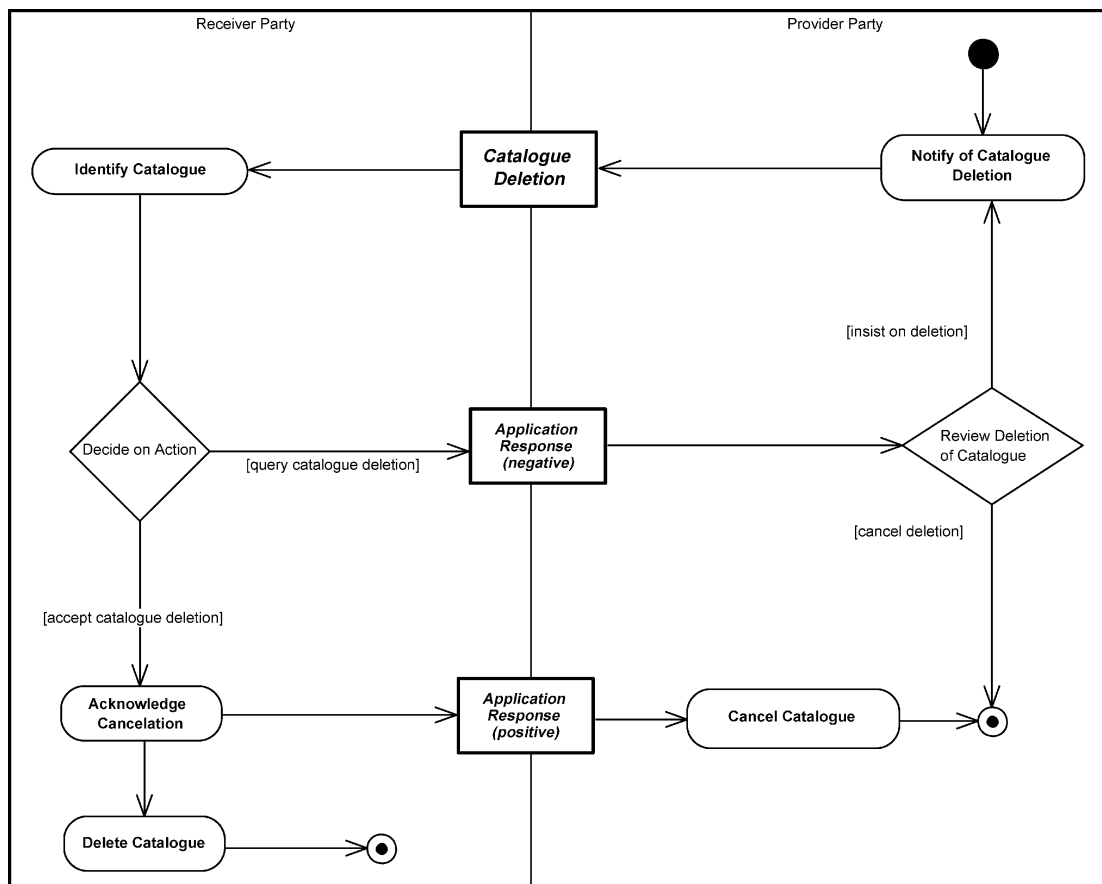
Figure 36 — Delete Catalogue Process
