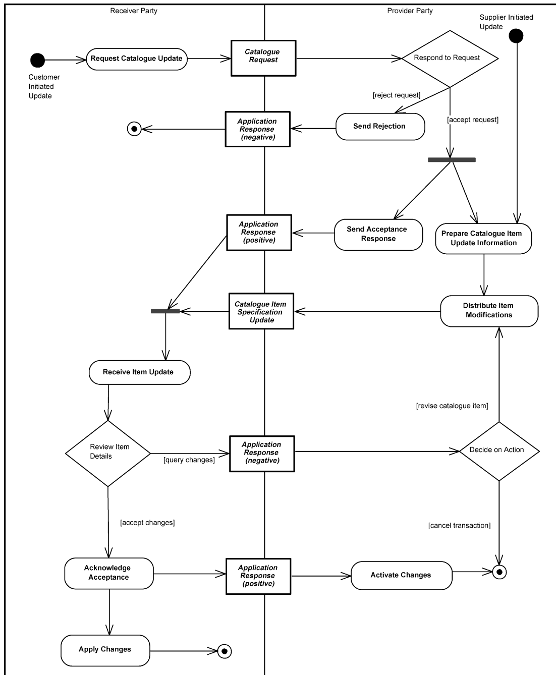
Figure 34 — Update Item Specification Process
