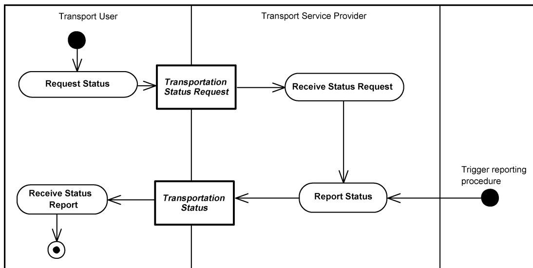
Figure 58 — Freight Status Reporting Process
