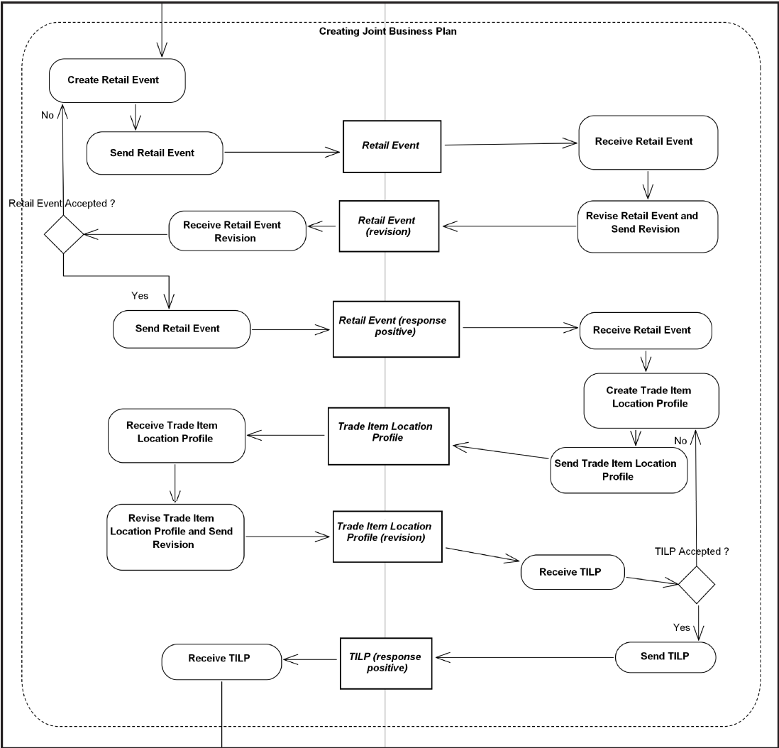
Figure 9 — Create Joint Business Plan
