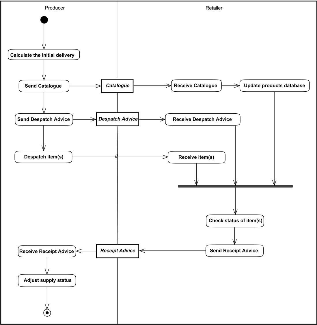
Figure 40 — Initial Stocking of the Area by Producer
