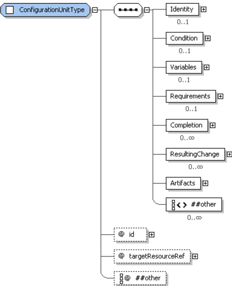
1372 1373 Figure 20: ConfigurationUnitType structure.
