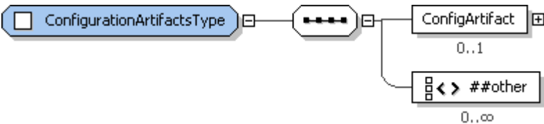
Figure 23: ConfigurationArtifactsType structure. ConfigurationArtifactsType provides the type definition for the Artifacts element of ConfigurationUnit .
