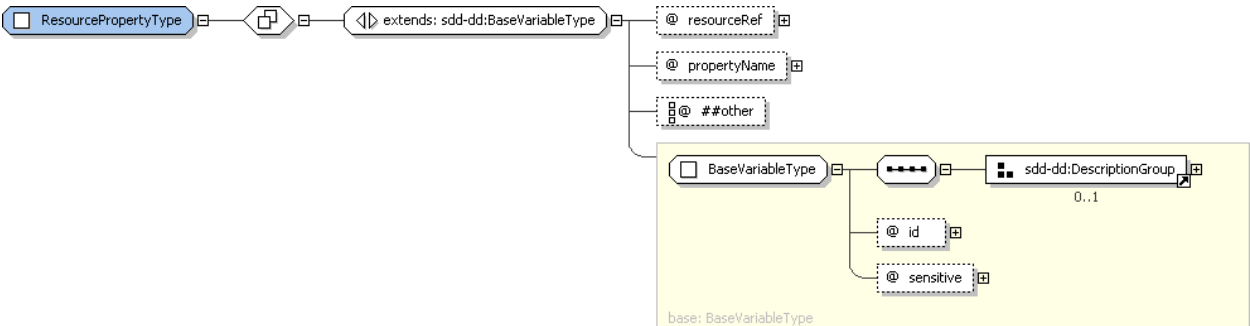
2283 2284 Figure 58: ResourcePropertyType structure.
