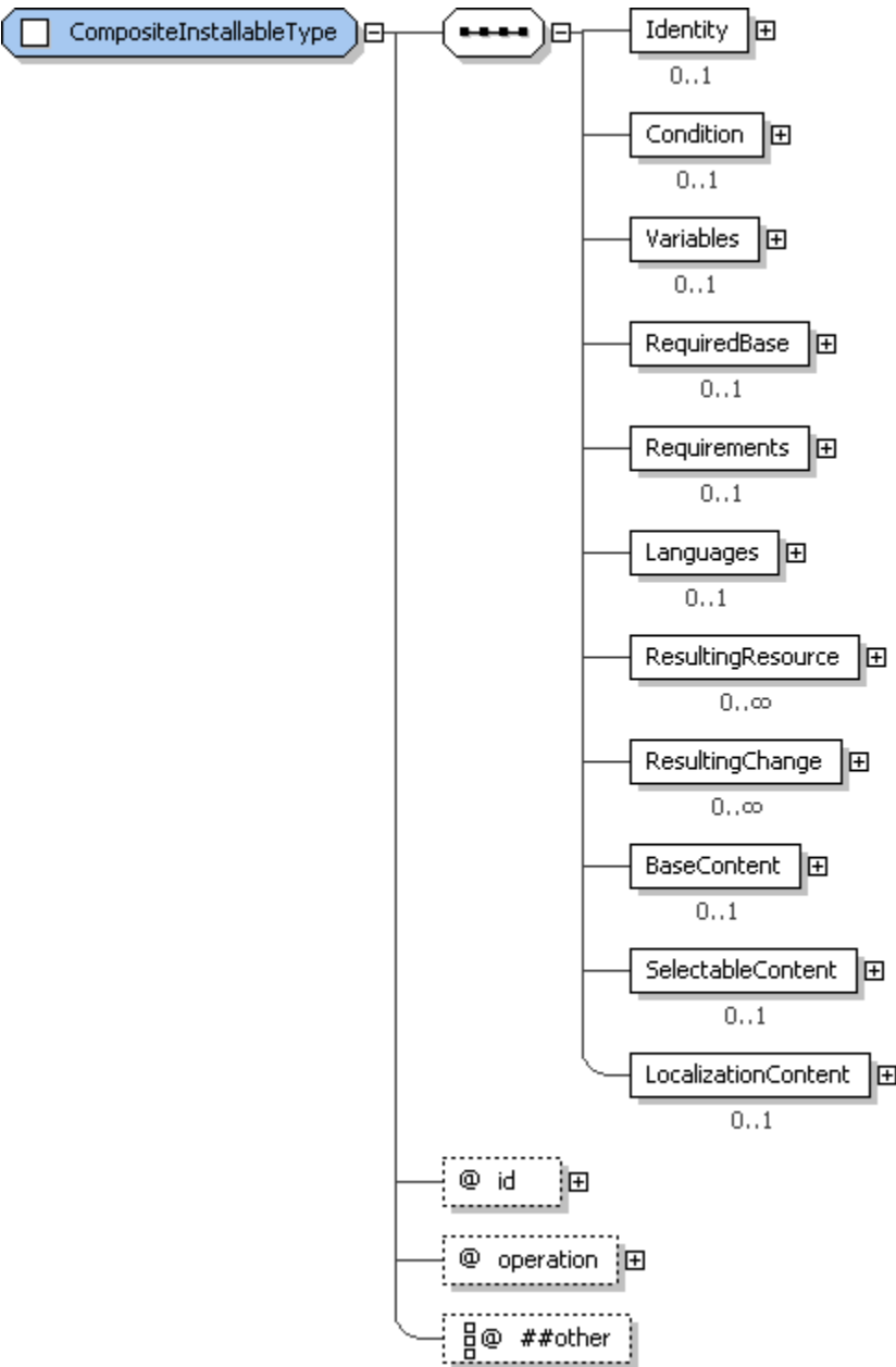
2789 Figure 73: CompositeInstallableType structure.
