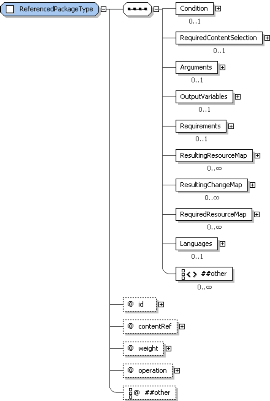
2959 Figure 78: ReferencedPackageType structure.
