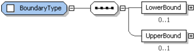
2232 Figure 54: BoundaryType structure.
