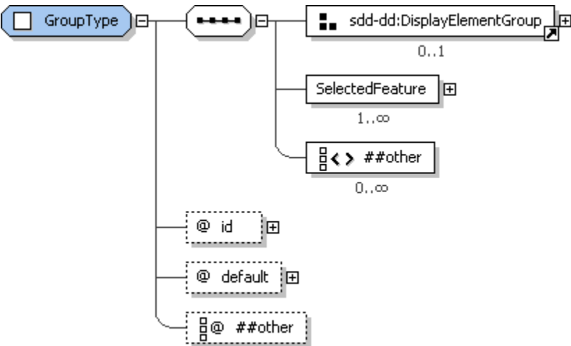
3267 3268 Figure 86: GroupType structure.
