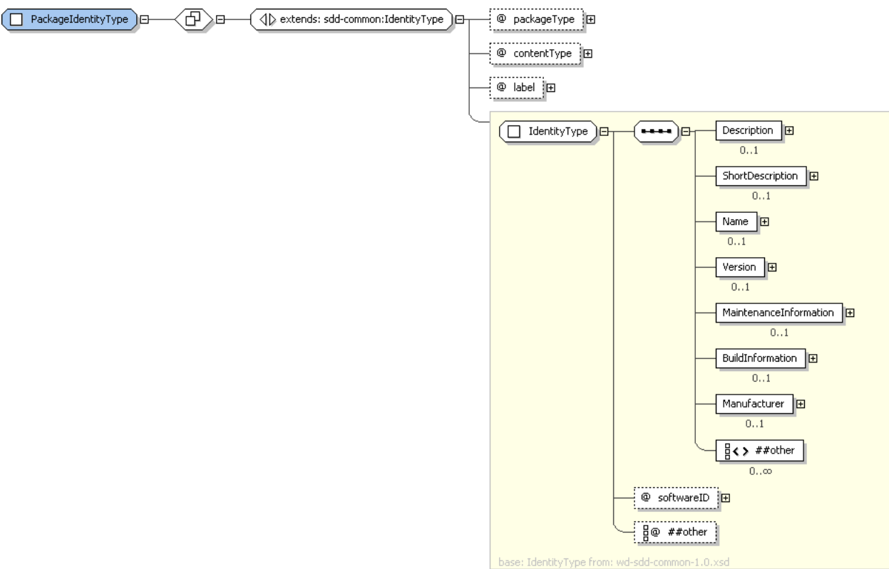
Figure 4: PackageIdentityType structure.
