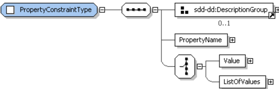
Figure 35: PropertyConstraintType structure.
