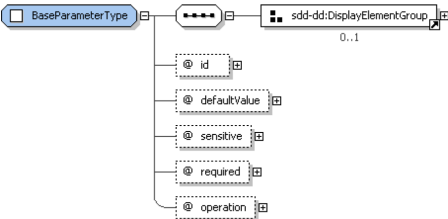
Figure 52: BaseParameterType structure.
