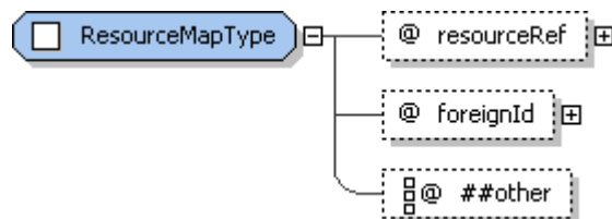
Figure 79: ResourceMapType structure.
