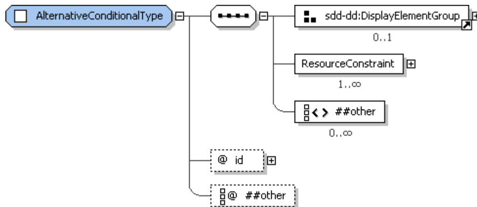
Figure 45: AlternativeConditionalType structure.
