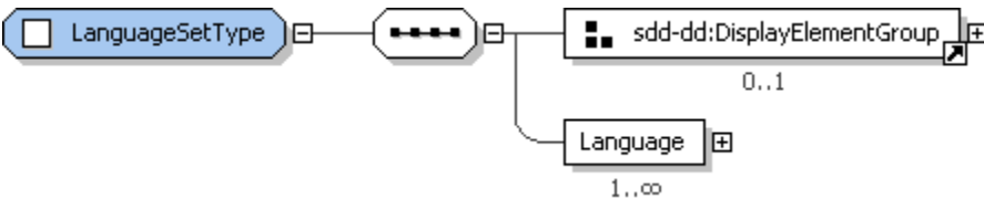
Figure 105: LanguageSetType structure.
