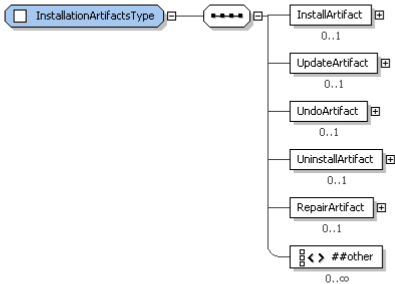
Figure 22: InstallationArtifactsType structure.
