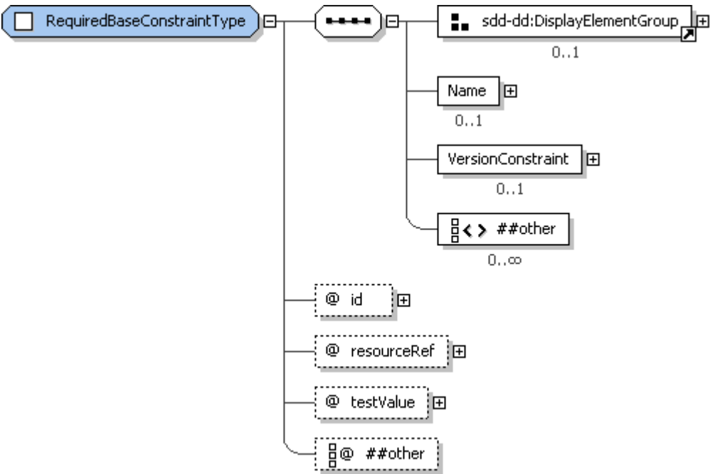
Figure 68: RequiredBaseConstraintType structure.
