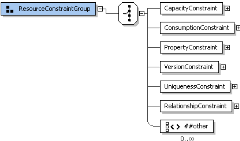
Figure 64: ResourceConstraintGroup structure.
