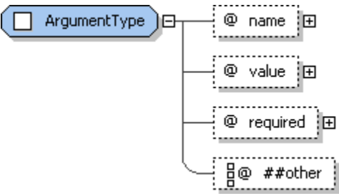
1561 1562 Figure 25: ArgumentType structure.
