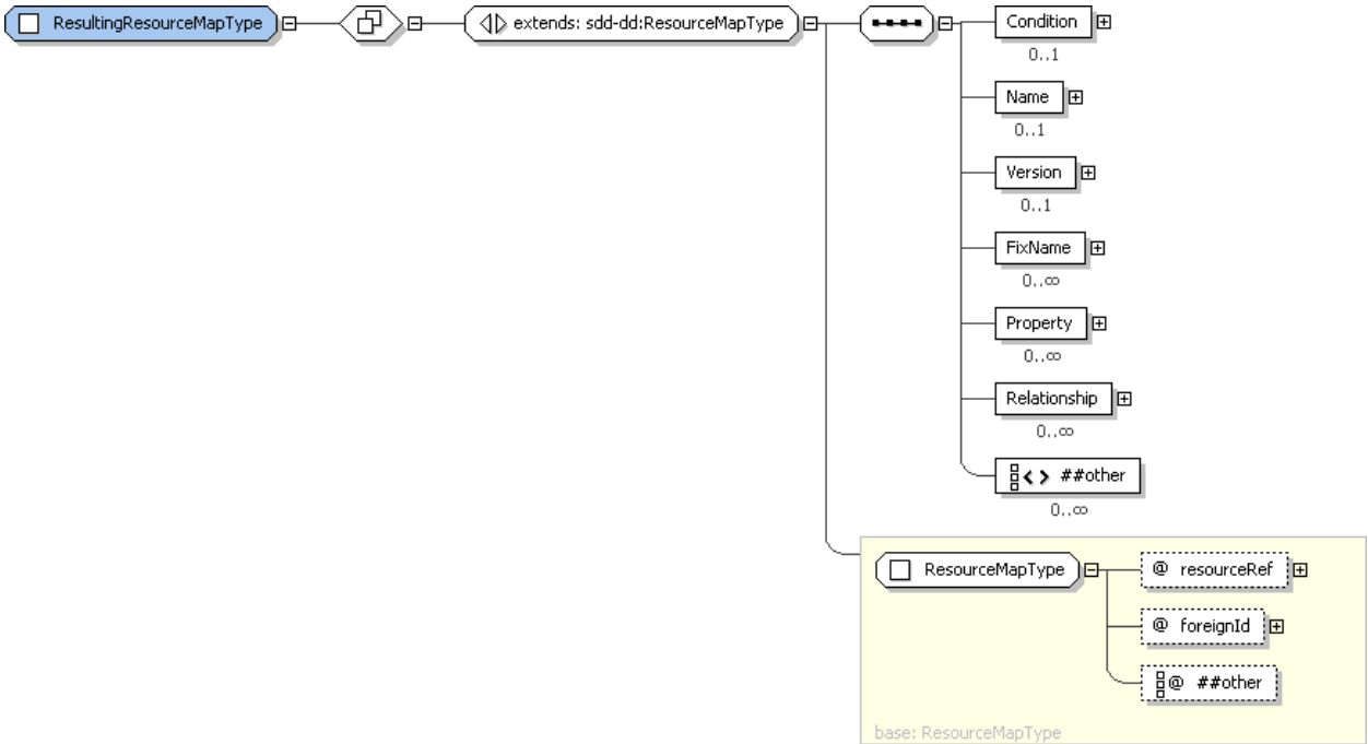
3093 3094 Figure 80: ResultingResourceMapType structure.
