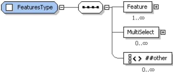
3289 3290 Figure 87: FeaturesType structure.
