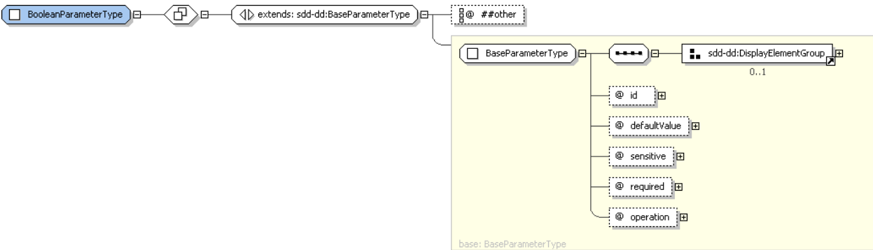
Figure 56: BooleanParameterType structure.
