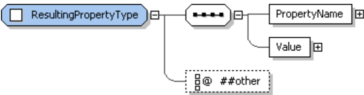
Figure 18: ResultingPropertyType structure.
