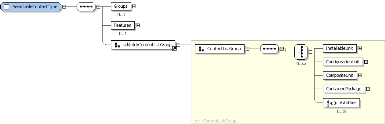
3229 3230 Figure 84: SelectableContentType structure.
