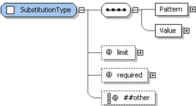
Figure 29: SubstitutionType structure.
