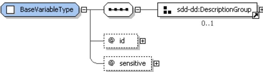
Figure 49: BaseVariableType structure.
