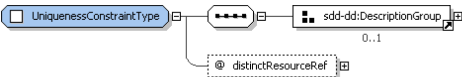
Figure 42: UniquenessConstraintType structure.
