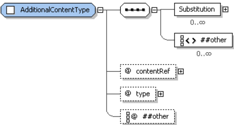
1599 Figure 28: AdditionalContentType structure.
