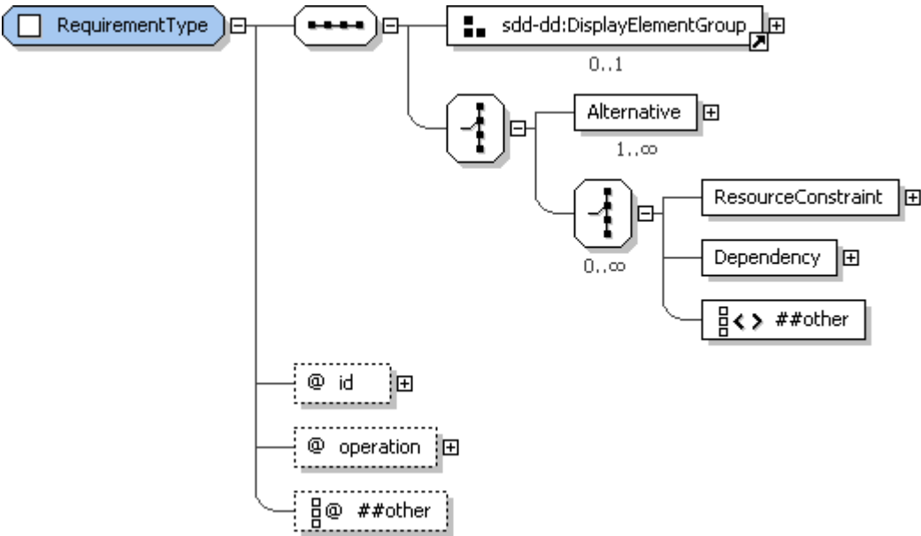
2360 2361 Figure 62: RequirementType structure.
