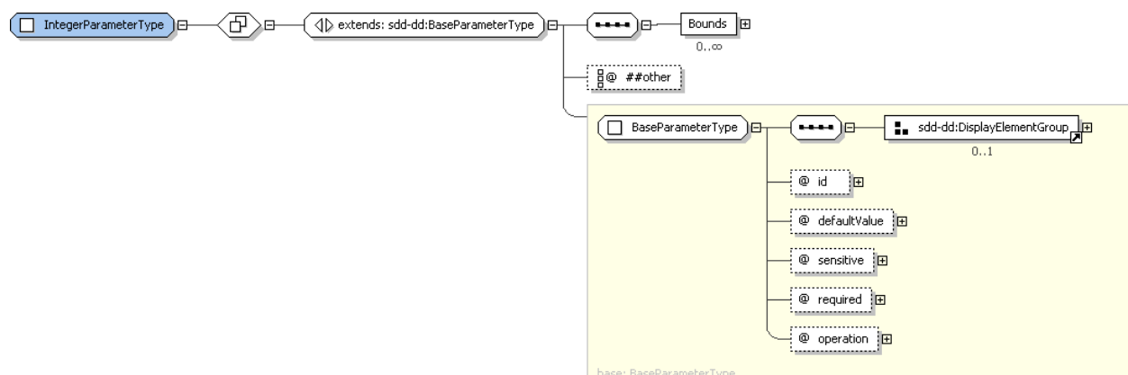
Figure 53: IntegerParameterType structure.
