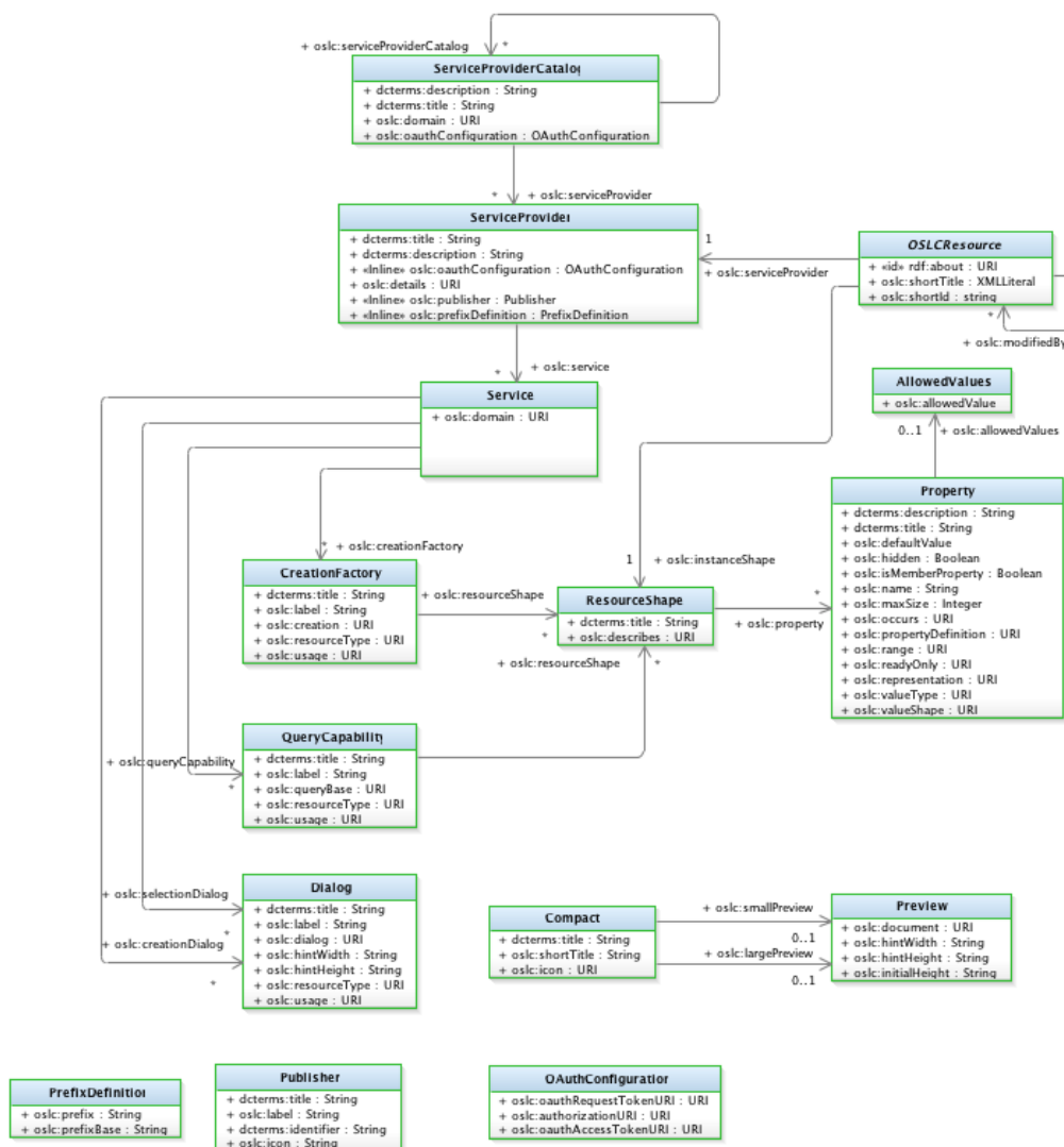
Fig. 1 Service Provider concepts and relationships
