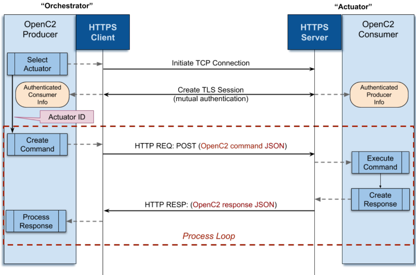
Figure 2 -- OpenC2 Consumer as HTTP Server
