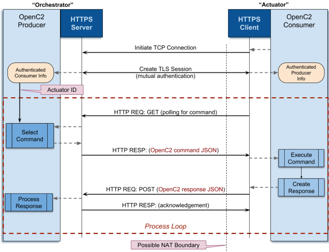
Figure 3 -- OpenC2 Producer as HTTP Server
