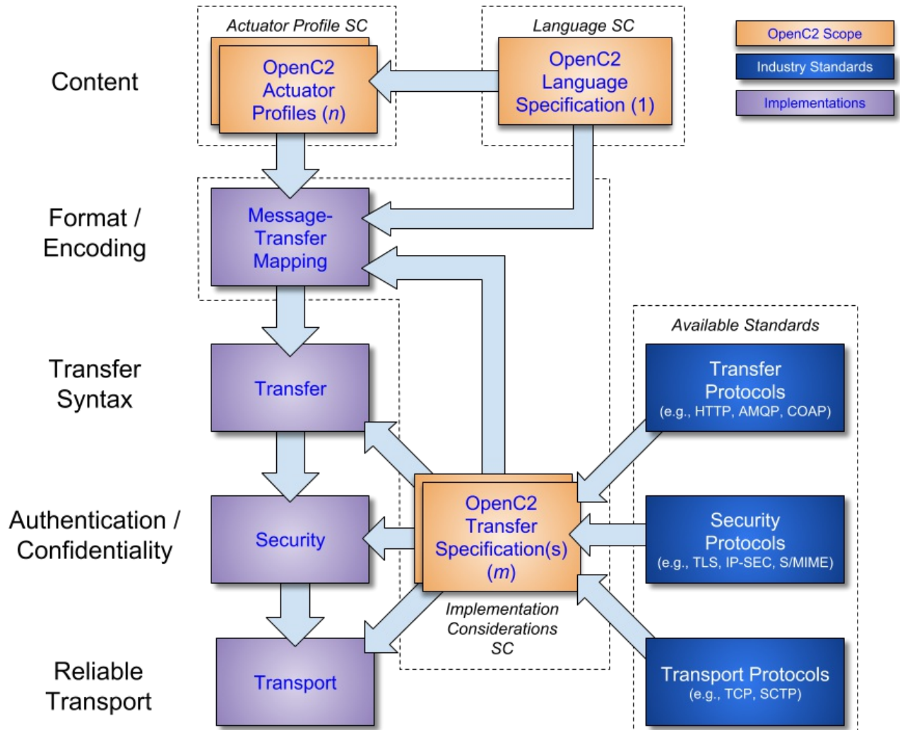
Figure 1 -- OpenC2 Documentation and Layering Model
