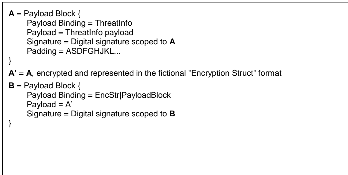
Figure 7 - Content Block Nesting of ThreatInfo Content
