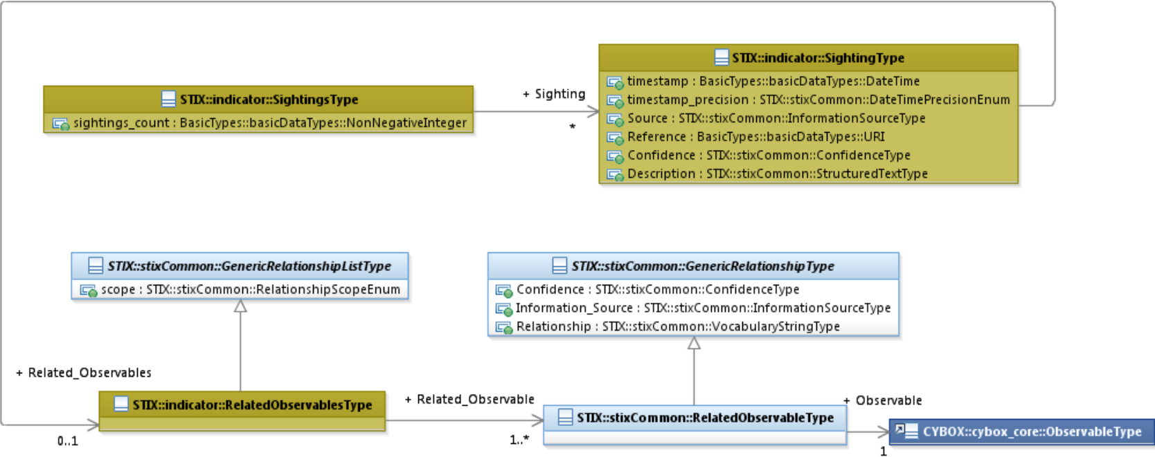
Figure 3-5. UML diagram of the RelatedObservablesType class The property table given in Table 3-12 corresponds to the UML diagram shown in Figure 3-5 . Table 3-12. Properties of the RelatedObservablesType class
