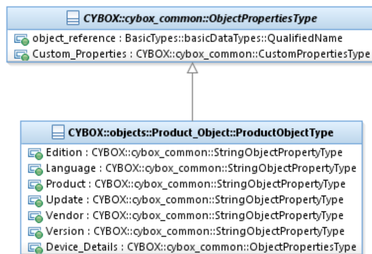
Figure 3-1. UML diagram of the ProductObjectType class
