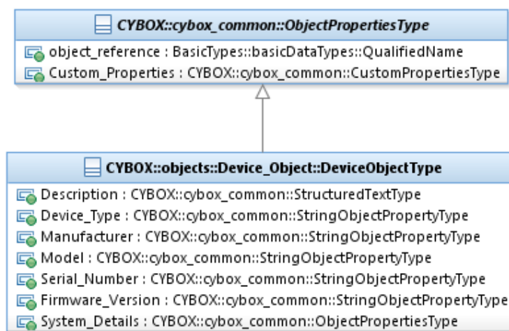
Figure 3-1. UML diagram of the DeviceObjectType class
