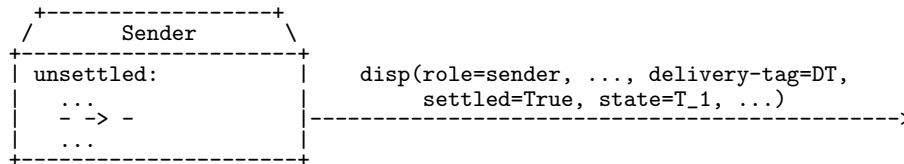
Figure 2.47: Indication of Settlement
