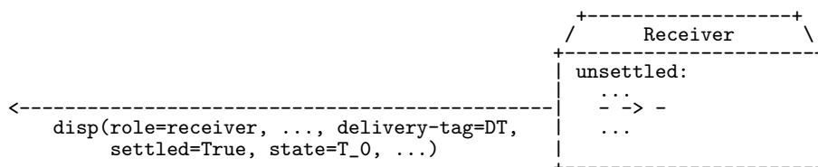
Figure 2.51: At-Least-Once
