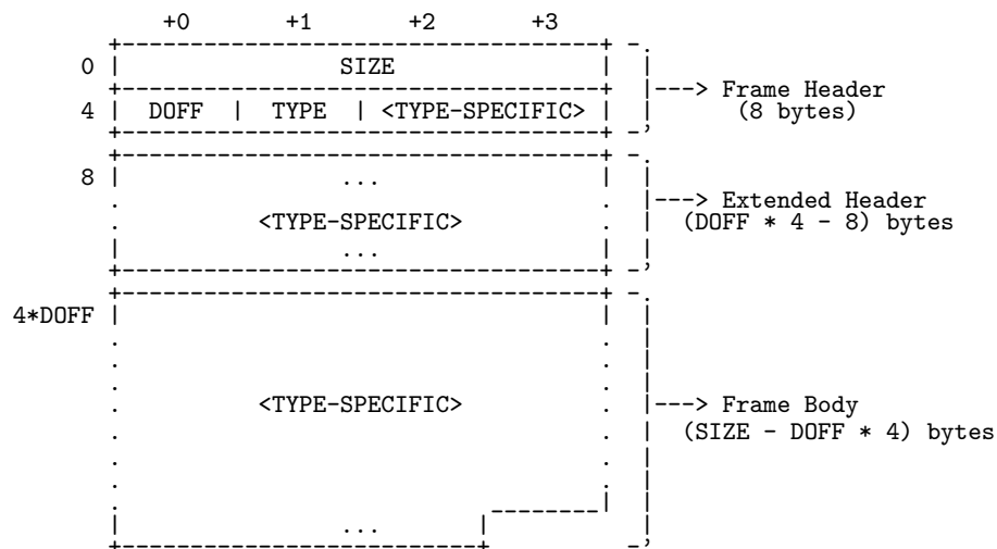
Figure 2.10: General Frame Layout
