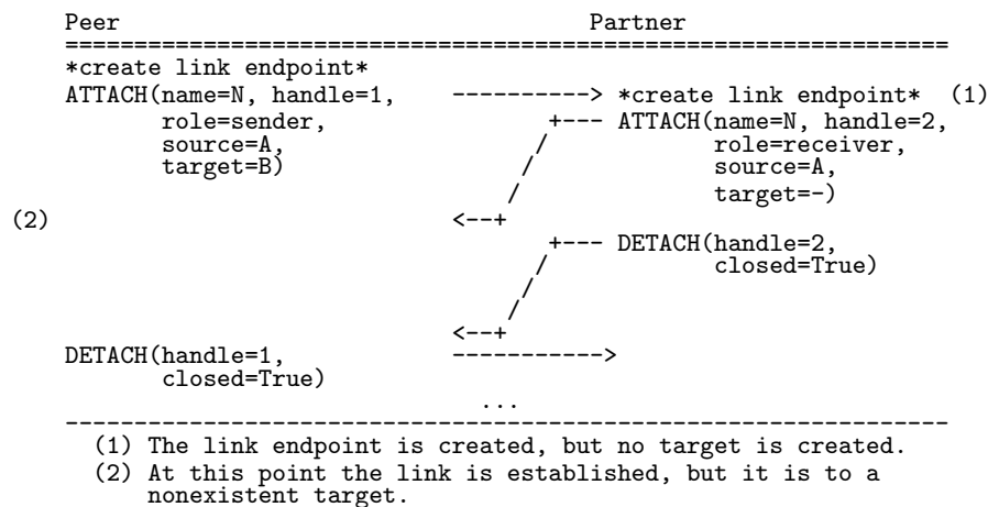
Figure 2.28: Refusing a Link
