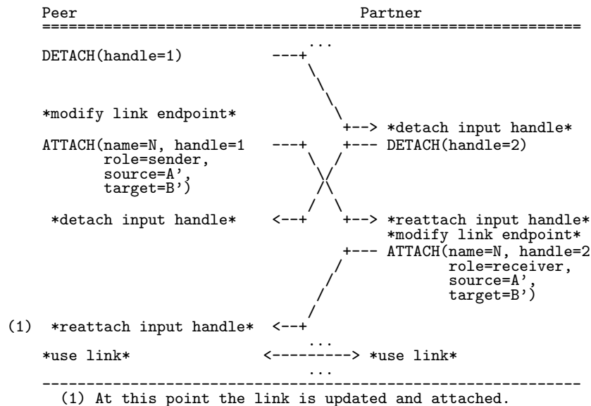
Figure 2.33: Updating Link State
