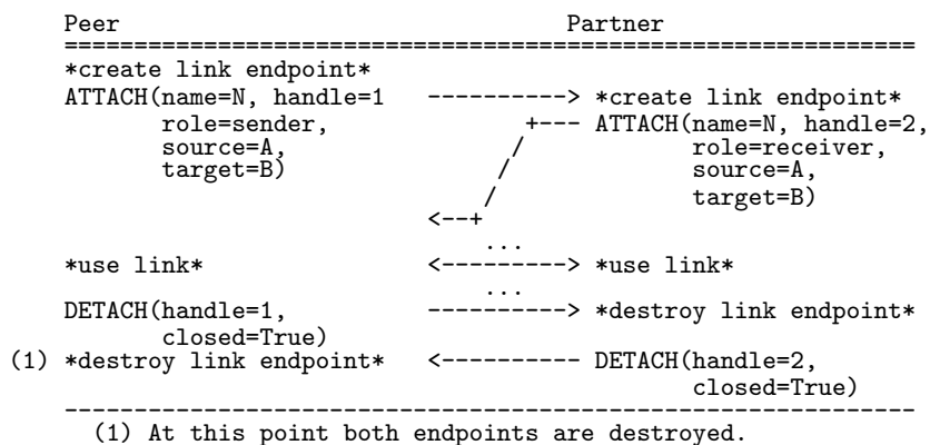
Figure 2.34: Closing a Link
