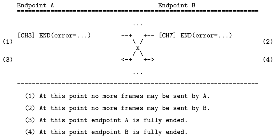
Figure 2.23: Simultaneous Session End Sequence
