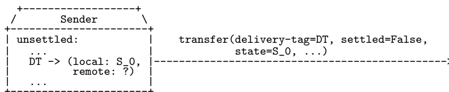
Figure 2.42: Initial Transfer
