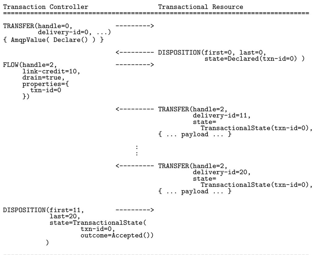
Figure 4.5: Transactional Acquisition
