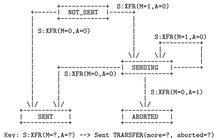
Figure 2.52: Outgoing Fragmentation State Diagram
