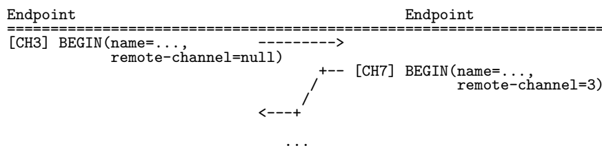
Figure 2.21: Session Begin Sequence
