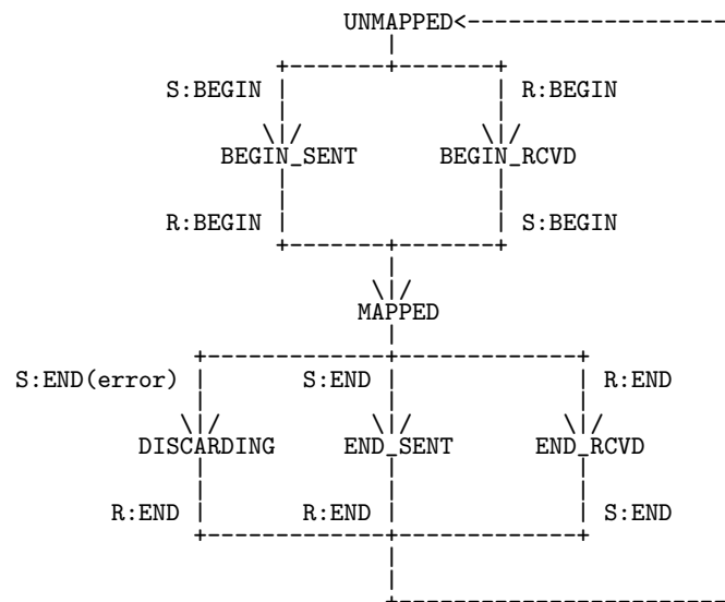
Figure 2.25: State Transitions
