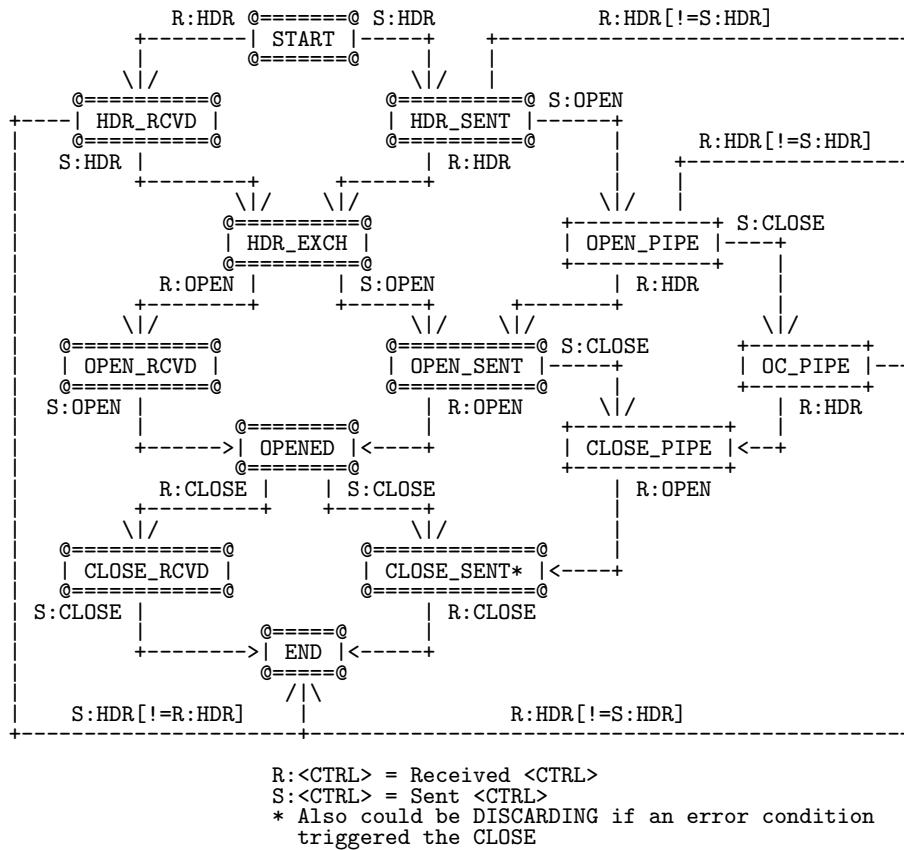
Figure 2.18: Connection State Diagram
