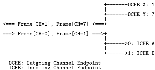
Figure 2.12: Unidirectional Channel Multiplexing
