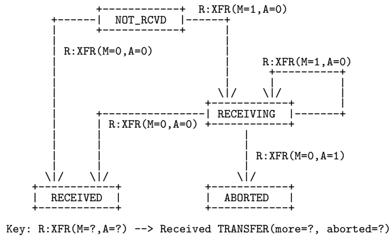
Figure 2.53: Incoming Fragmentation State Diagram
