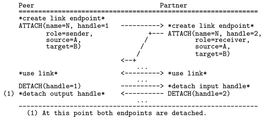
Figure 2.32: Detaching a Link
