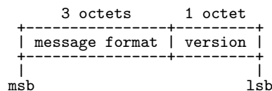
Figure 2.54: Layout of Message Format Code
