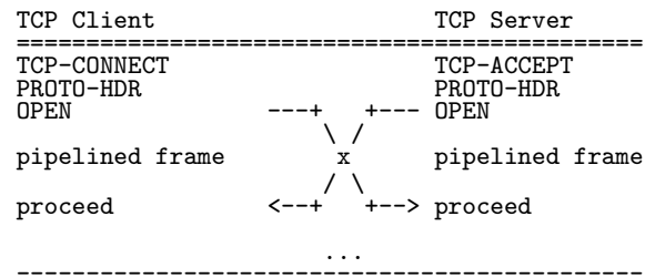
Figure 2.15: Pipelined Connection Open Sequence
