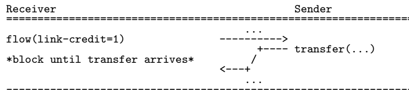
Figure 2.38: Synchronous Get
