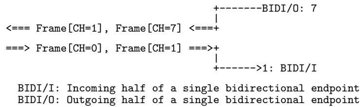
Figure 2.13: Bidirectional Channel Multiplexing
