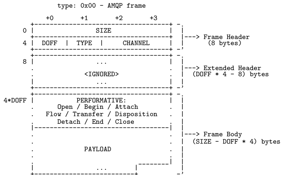
Figure 2.11: AMQP Frame Layout
