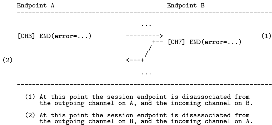
Figure 2.22: Session End Sequence
