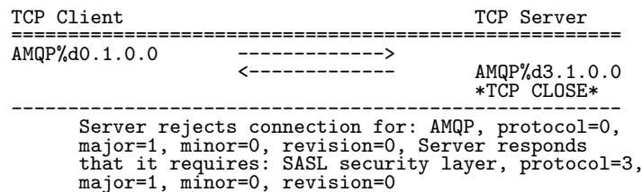
Figure 2.8: Protocol ID Rejection Example
